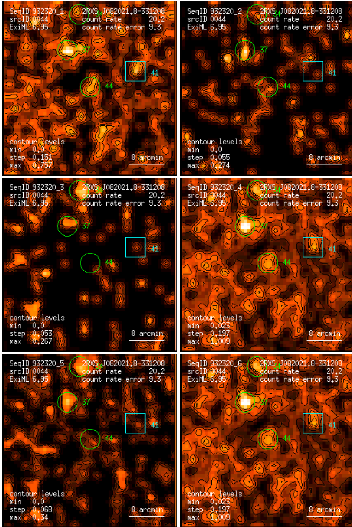
Figure 44: RASS 932320: detection 0044: band rate images, Gaussian filter: (1) PSPC channels 11 – 41, (2) 52 – 90, (3) 91 – 201, (4) 11 – 235, (5) 52 – 201, (6) 11 – 201. Broad band rates in counts/ks. Band rate contour levels in counts/ks/arcmin 2 .
