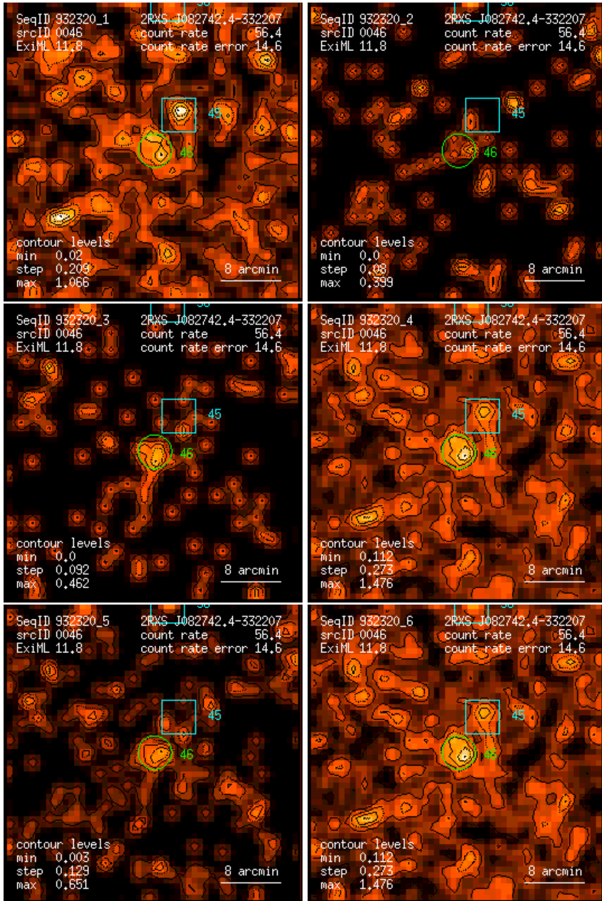
Figure 46: RASS 932320: detection 0046: band rate images, Gaussian filter: (1) PSPC channels 11 – 41, (2) 52 – 90, (3) 91 – 201, (4) 11 – 235, (5) 52 – 201, (6) 11 – 201. Broad band rates in counts/ks. Band rate contour levels in counts/ks/arcmin 2 .
