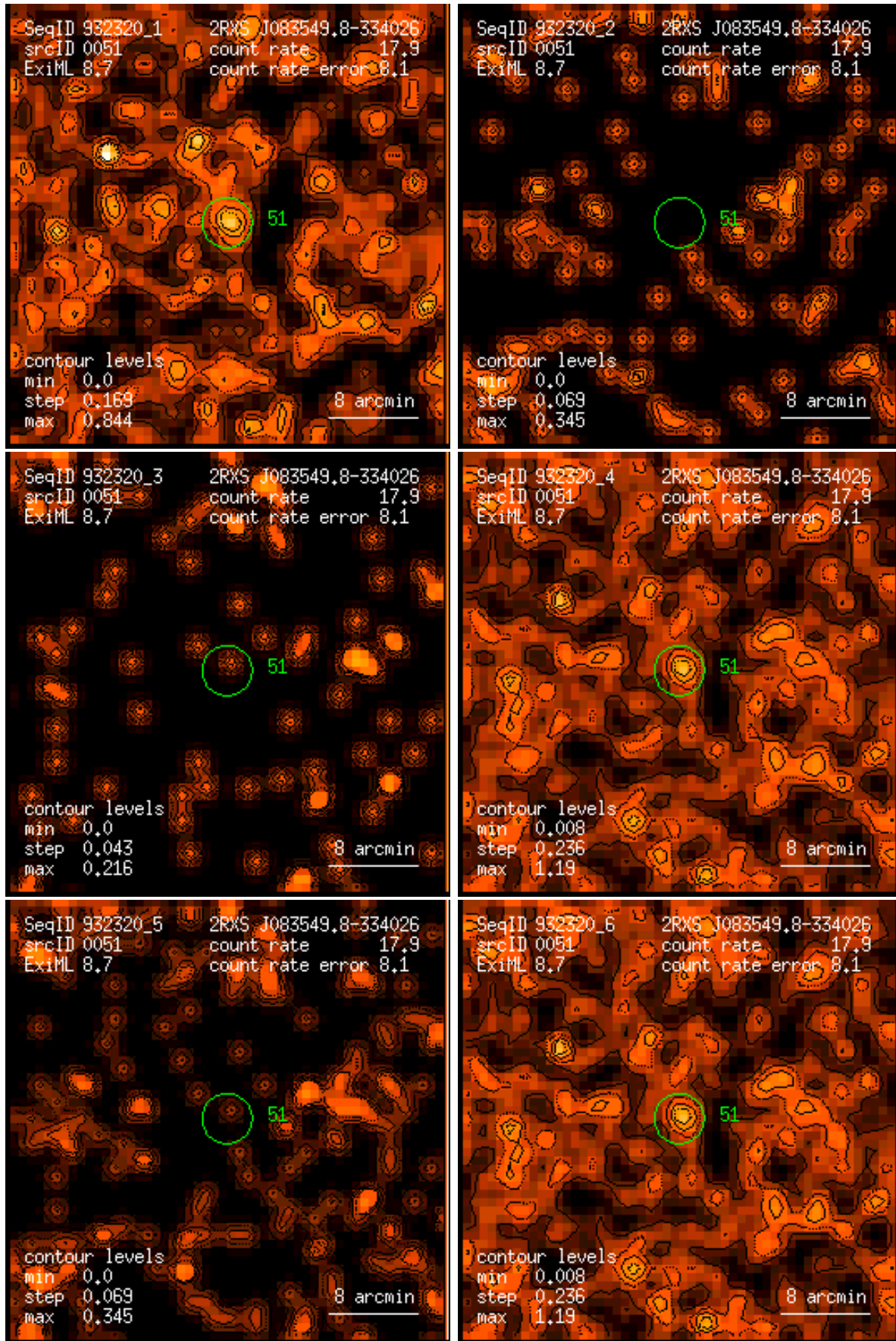
Figure 51: RASS 932320: detection 0051: band rate images, Gaussian filter: (1) PSPC channels 11 – 41, (2) 52 – 90, (3) 91 – 201, (4) 11 – 235, (5) 52 – 201, (6) 11 – 201. Broad band rates in counts/ks. Band rate contour levels in counts/ks/arcmin 2 .
