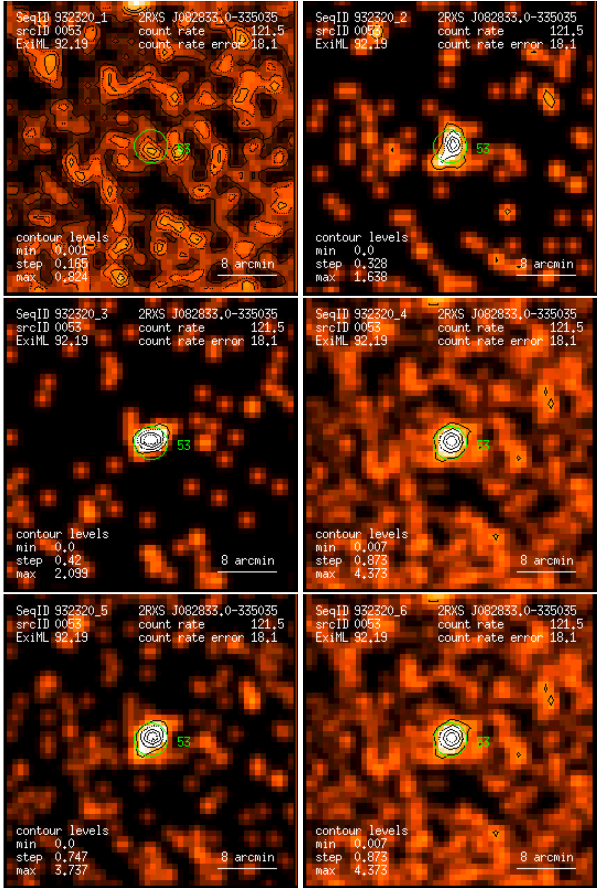
Figure 53: RASS 932320: detection 0053: band rate images, Gaussian filter: (1) PSPC channels 11 – 41, (2) 52 – 90, (3) 91 – 201, (4) 11 – 235, (5) 52 – 201, (6) 11 – 201. Broad band rates in counts/ks. Band rate contour levels in counts/ks/arcmin 2 .
