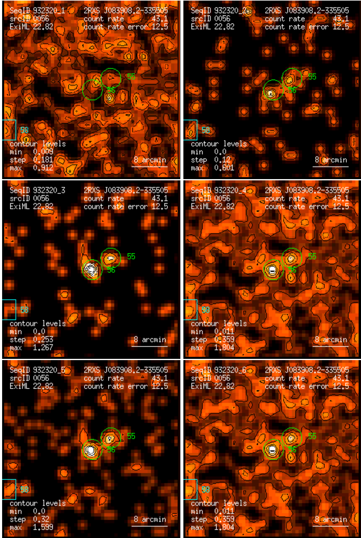
Figure 56: RASS 932320: detection 0056: band rate images, Gaussian filter: (1) PSPC channels 11 – 41, (2) 52 – 90, (3) 91 – 201, (4) 11 – 235, (5) 52 – 201, (6) 11 – 201. Broad band rates in counts/ks. Band rate contour levels in counts/ks/arcmin 2 .
