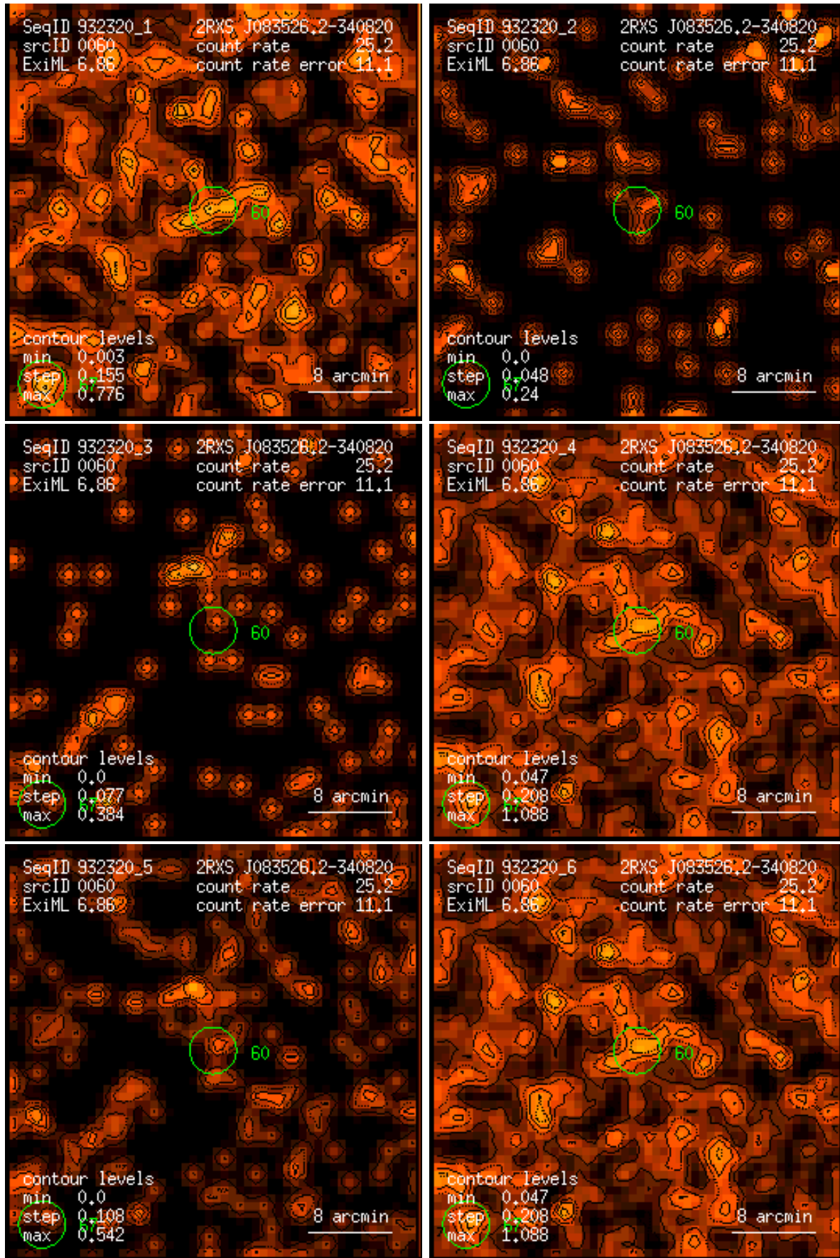
Figure 60: RASS 932320: detection 0060: band rate images, Gaussian filter: (1) PSPC channels 11 – 41, (2) 52 – 90, (3) 91 – 201, (4) 11 – 235, (5) 52 – 201, (6) 11 – 201. Broad band rates in counts/ks. Band rate contour levels in counts/ks/arcmin 2 .
