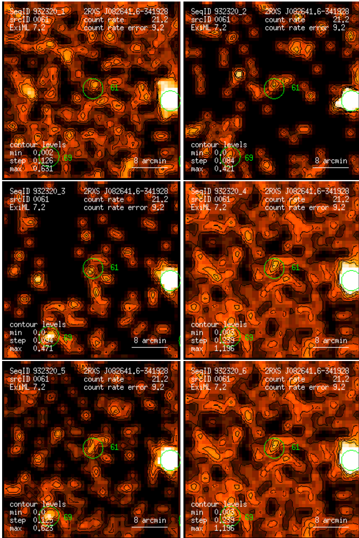
Figure 61: RASS 932320: detection 0061: band rate images, Gaussian filter: (1) PSPC channels 11 – 41, (2) 52 – 90, (3) 91 – 201, (4) 11 – 235, (5) 52 – 201, (6) 11 – 201. Broad band rates in counts/ks. Band rate contour levels in counts/ks/arcmin 2 .
