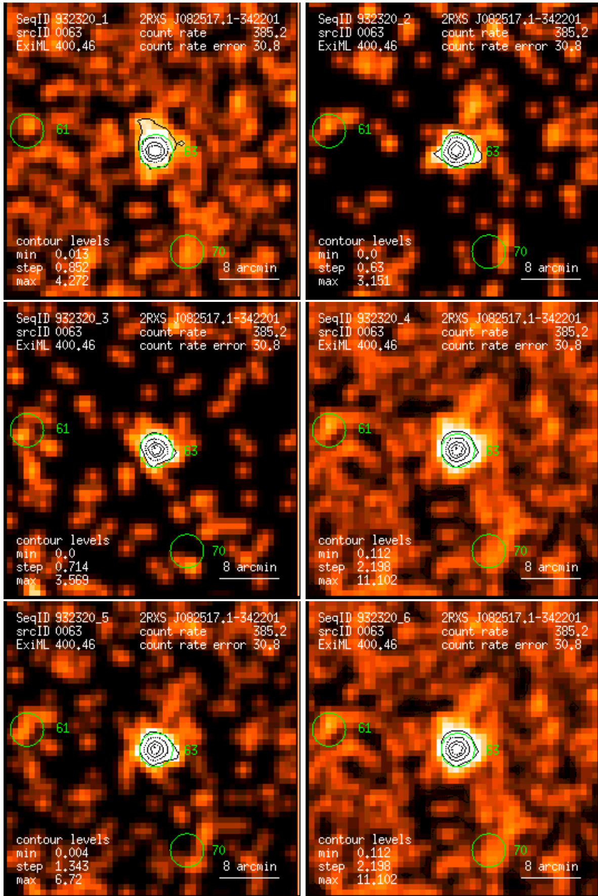
Figure 63: RASS 932320: detection 0063: band rate images, Gaussian filter: (1) PSPC channels 11 – 41, (2) 52 – 90, (3) 91 – 201, (4) 11 – 235, (5) 52 – 201, (6) 11 – 201. Broad band rates in counts/ks. Band rate contour levels in counts/ks/arcmin 2 .
