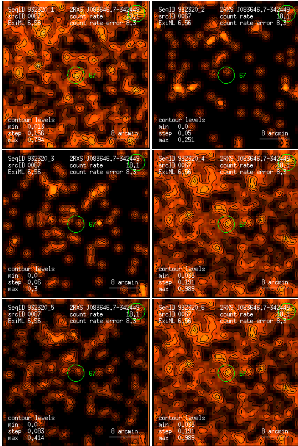
Figure 67: RASS 932320: detection 0067: band rate images, Gaussian filter: (1) PSPC channels 11 – 41, (2) 52 – 90, (3) 91 – 201, (4) 11 – 235, (5) 52 – 201, (6) 11 – 201. Broad band rates in counts/ks. Band rate contour levels in counts/ks/arcmin 2 .
