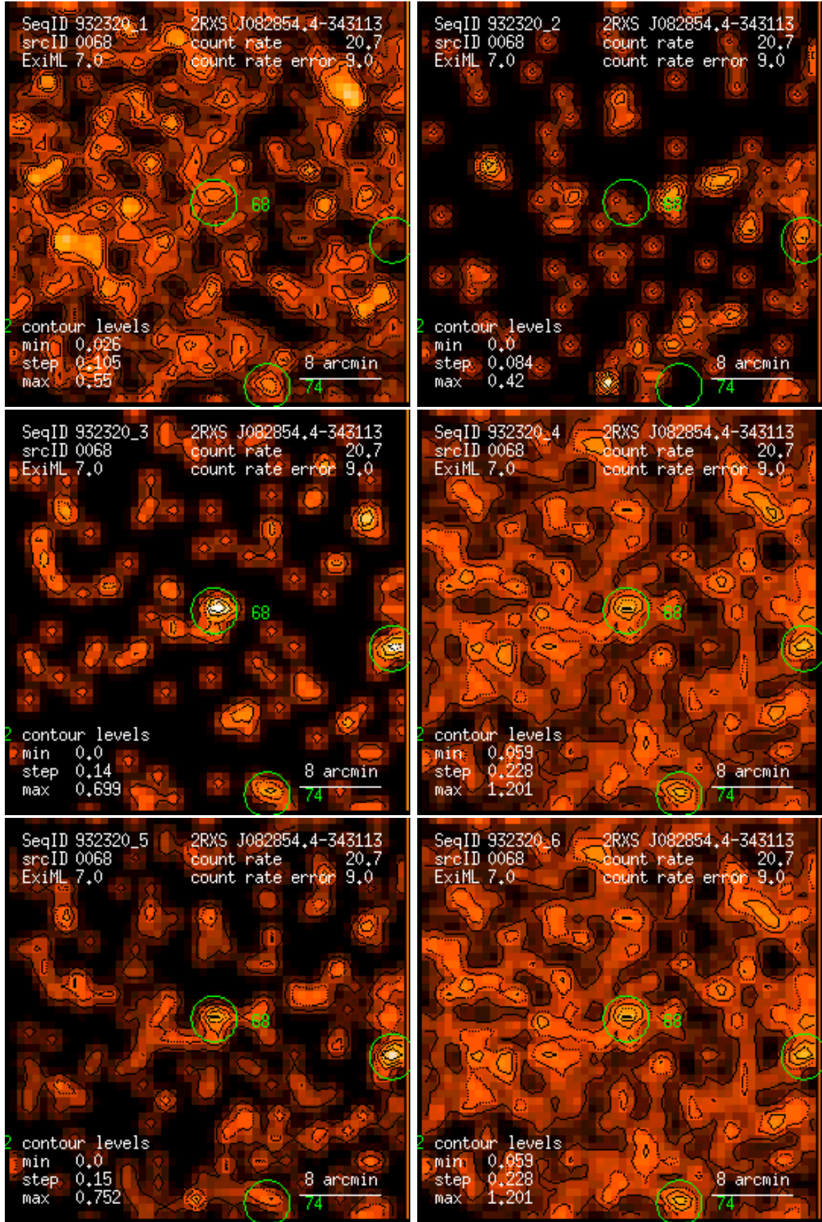
Figure 68: RASS 932320: detection 0068: band rate images, Gaussian filter: (1) PSPC channels 11 – 41, (2) 52 – 90, (3) 91 – 201, (4) 11 – 235, (5) 52 – 201, (6) 11 – 201. Broad band rates in counts/ks. Band rate contour levels in counts/ks/arcmin 2 .
