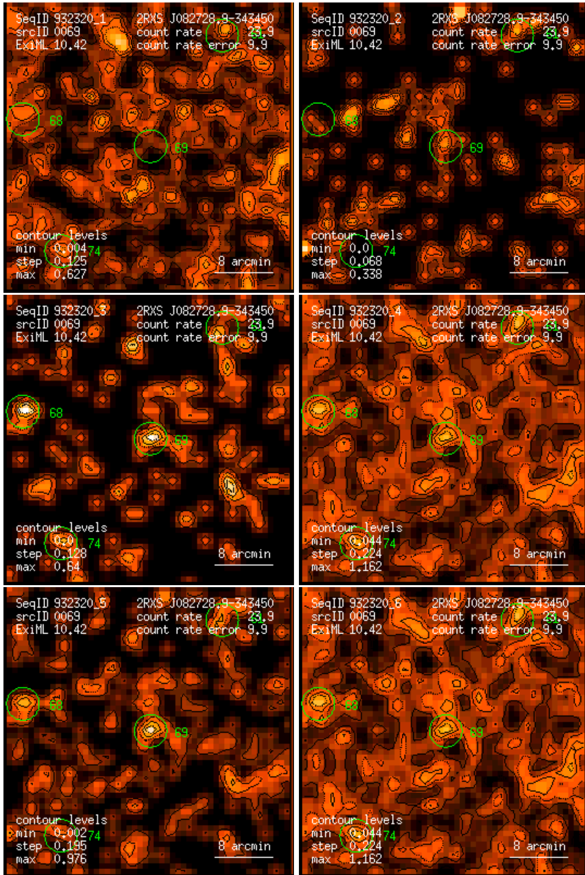
Figure 69: RASS 932320: detection 0069: band rate images, Gaussian filter: (1) PSPC channels 11 – 41, (2) 52 – 90, (3) 91 – 201, (4) 11 – 235, (5) 52 – 201, (6) 11 – 201. Broad band rates in counts/ks. Band rate contour levels in counts/ks/arcmin 2 .
