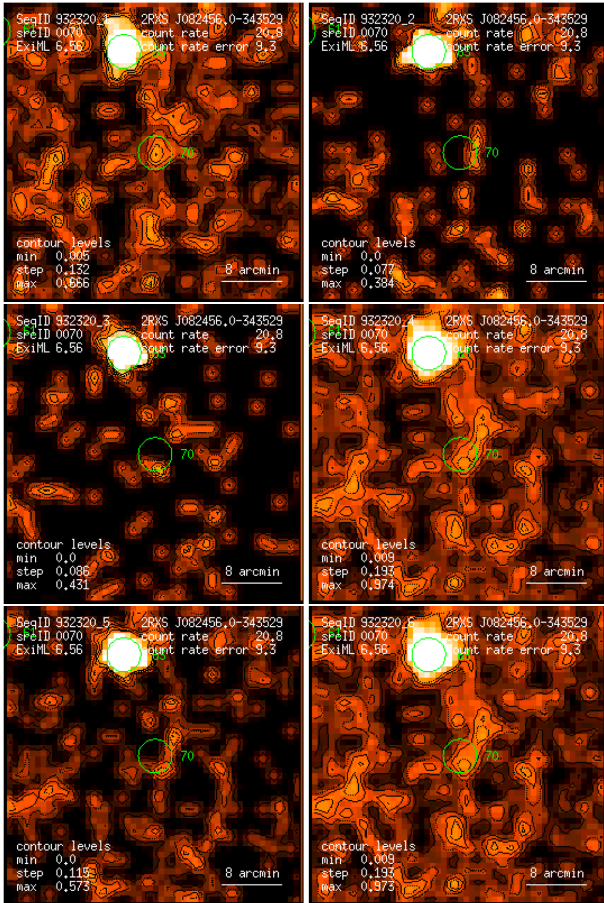
Figure 70: RASS 932320: detection 0070: band rate images, Gaussian filter: (1) PSPC channels 11 – 41, (2) 52 – 90, (3) 91 – 201, (4) 11 – 235, (5) 52 – 201, (6) 11 – 201. Broad band rates in counts/ks. Band rate contour levels in counts/ks/arcmin 2 .
