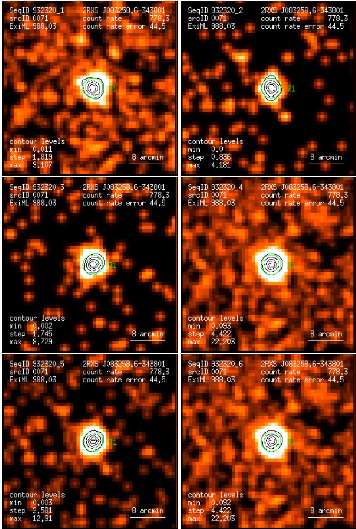
Figure 71: RASS 932320: detection 0071: band rate images, Gaussian filter: (1) PSPC channels 11 – 41, (2) 52 – 90, (3) 91 – 201, (4) 11 – 235, (5) 52 – 201, (6) 11 – 201. Broad band rates in counts/ks. Band rate contour levels in counts/ks/arcmin 2 .
