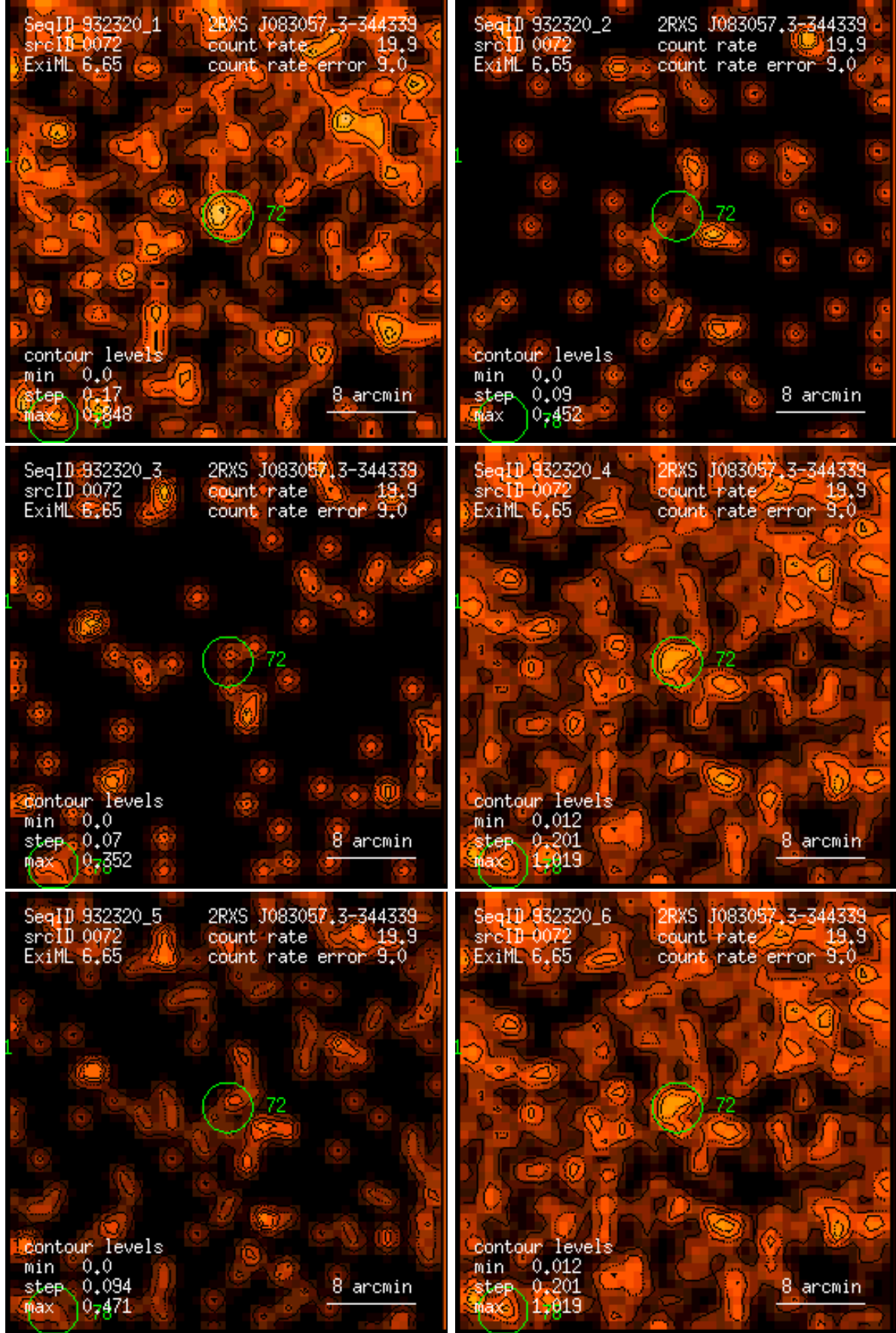
Figure 72: RASS 932320: detection 0072: band rate images, Gaussian filter: (1) PSPC channels 11 – 41, (2) 52 – 90, (3) 91 – 201, (4) 11 – 235, (5) 52 – 201, (6) 11 – 201. Broad band rates in counts/ks. Band rate contour levels in counts/ks/arcmin 2 .
