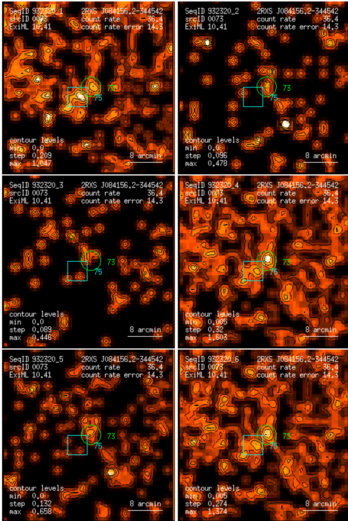
Figure 73: RASS 932320: detection 0073: band rate images, Gaussian filter: (1) PSPC channels 11 – 41, (2) 52 – 90, (3) 91 – 201, (4) 11 – 235, (5) 52 – 201, (6) 11 – 201. Broad band rates in counts/ks. Band rate contour levels in counts/ks/arcmin 2 .
