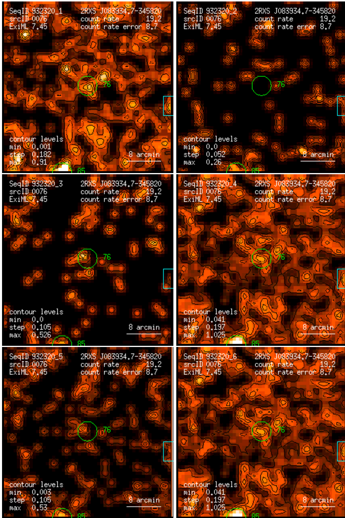
Figure 76: RASS 932320: detection 0076: band rate images, Gaussian filter: (1) PSPC channels 11 – 41, (2) 52 – 90, (3) 91 – 201, (4) 11 – 235, (5) 52 – 201, (6) 11 – 201. Broad band rates in counts/ks. Band rate contour levels in counts/ks/arcmin 2 .
