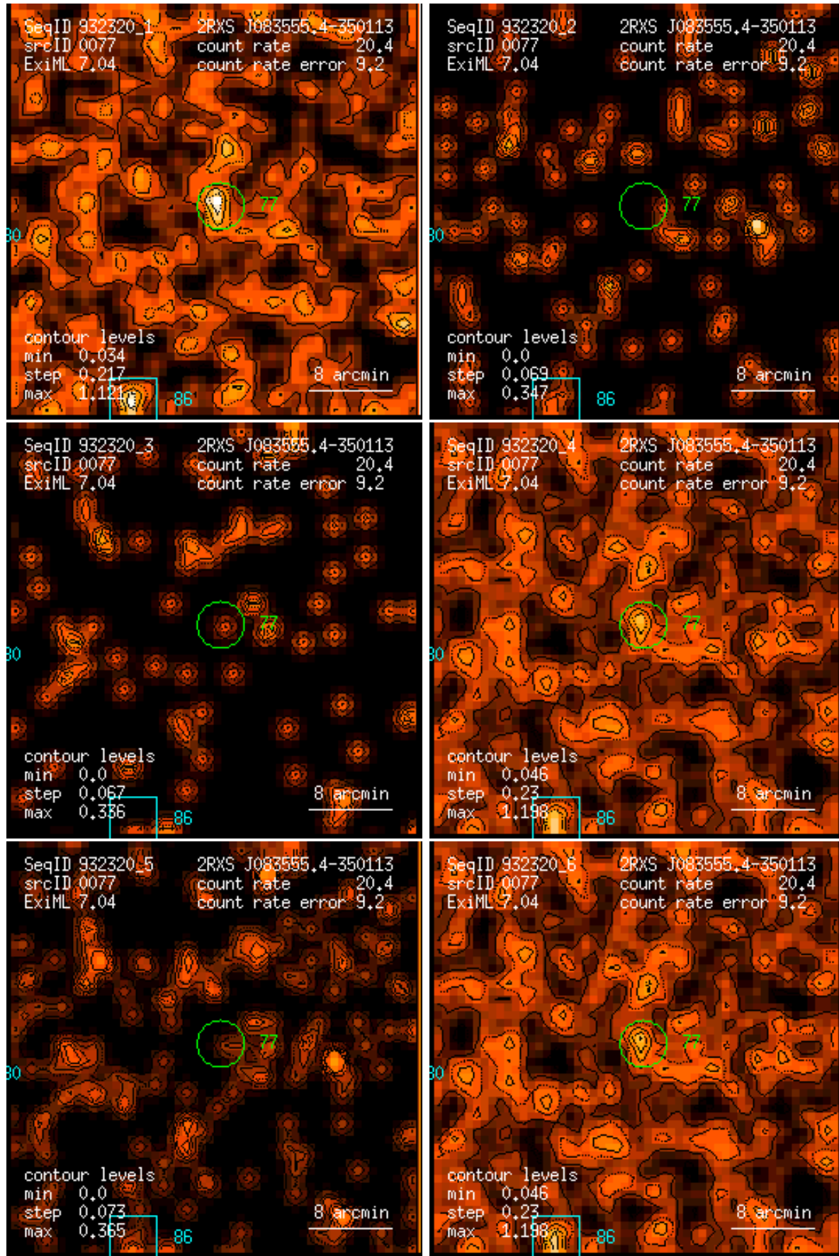
Figure 77: RASS 932320: detection 0077: band rate images, Gaussian filter: (1) PSPC channels 11 – 41, (2) 52 – 90, (3) 91 – 201, (4) 11 – 235, (5) 52 – 201, (6) 11 – 201. Broad band rates in counts/ks. Band rate contour levels in counts/ks/arcmin 2 .
