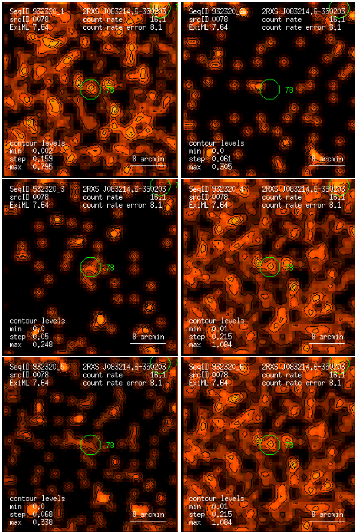
Figure 78: RASS 932320: detection 0078: band rate images, Gaussian filter: (1) PSPC channels 11 – 41, (2) 52 – 90, (3) 91 – 201, (4) 11 – 235, (5) 52 – 201, (6) 11 – 201. Broad band rates in counts/ks. Band rate contour levels in counts/ks/arcmin 2 .
