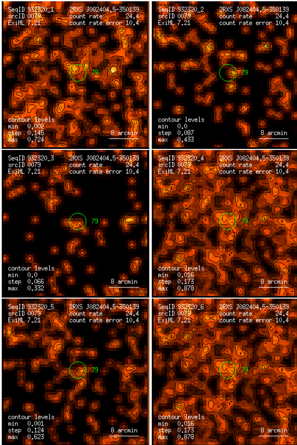
Figure 79: RASS 932320: detection 0079: band rate images, Gaussian filter: (1) PSPC channels 11 – 41, (2) 52 – 90, (3) 91 – 201, (4) 11 – 235, (5) 52 – 201, (6) 11 – 201. Broad band rates in counts/ks. Band rate contour levels in counts/ks/arcmin 2 .
