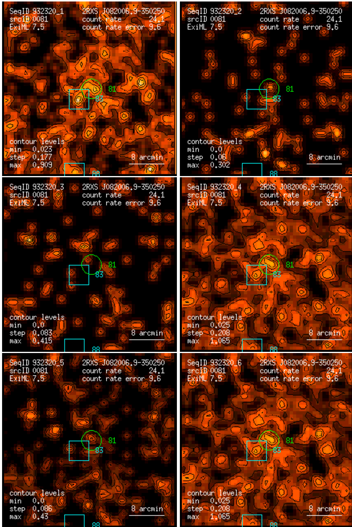
Figure 81: RASS 932320: detection 0081: band rate images, Gaussian filter: (1) PSPC channels 11 – 41, (2) 52 – 90, (3) 91 – 201, (4) 11 – 235, (5) 52 – 201, (6) 11 – 201. Broad band rates in counts/ks. Band rate contour levels in counts/ks/arcmin 2 .
