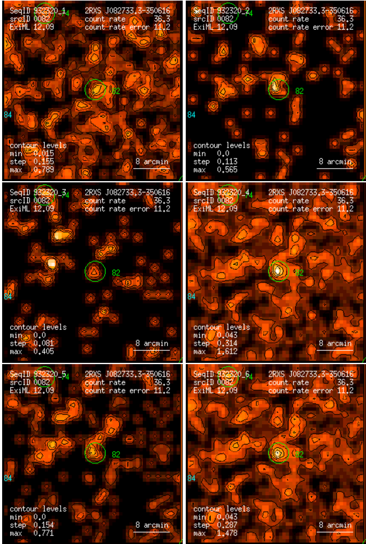
Figure 82: RASS 932320: detection 0082: band rate images, Gaussian filter: (1) PSPC channels 11 – 41, (2) 52 – 90, (3) 91 – 201, (4) 11 – 235, (5) 52 – 201, (6) 11 – 201. Broad band rates in counts/ks. Band rate contour levels in counts/ks/arcmin 2 .
