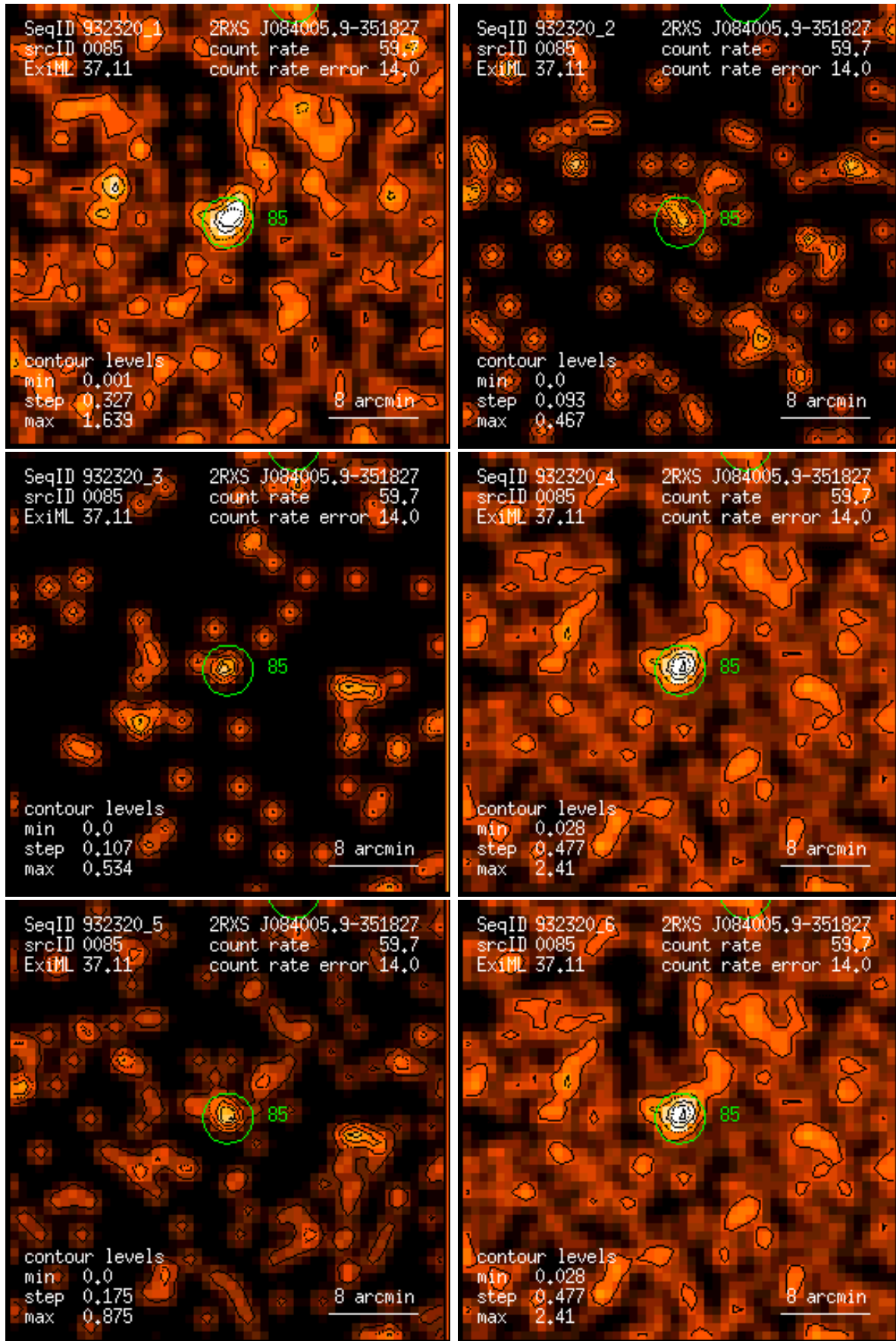
Figure 85: RASS 932320: detection 0085: band rate images, Gaussian filter: (1) PSPC channels 11 – 41, (2) 52 – 90, (3) 91 – 201, (4) 11 – 235, (5) 52 – 201, (6) 11 – 201. Broad band rates in counts/ks. Band rate contour levels in counts/ks/arcmin 2 .
