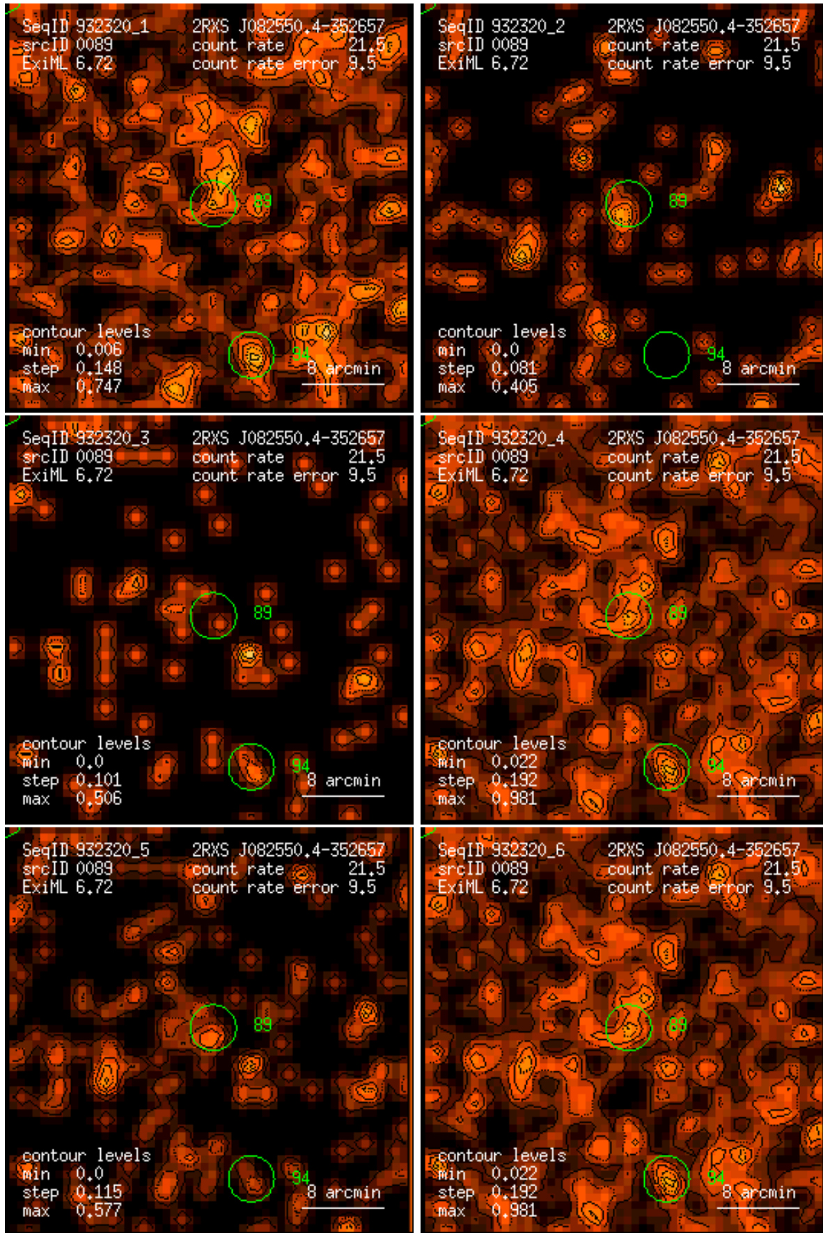
Figure 89: RASS 932320: detection 0089: band rate images, Gaussian filter: (1) PSPC channels 11 – 41, (2) 52 – 90, (3) 91 – 201, (4) 11 – 235, (5) 52 – 201, (6) 11 – 201. Broad band rates in counts/ks. Band rate contour levels in counts/ks/arcmin 2 .
