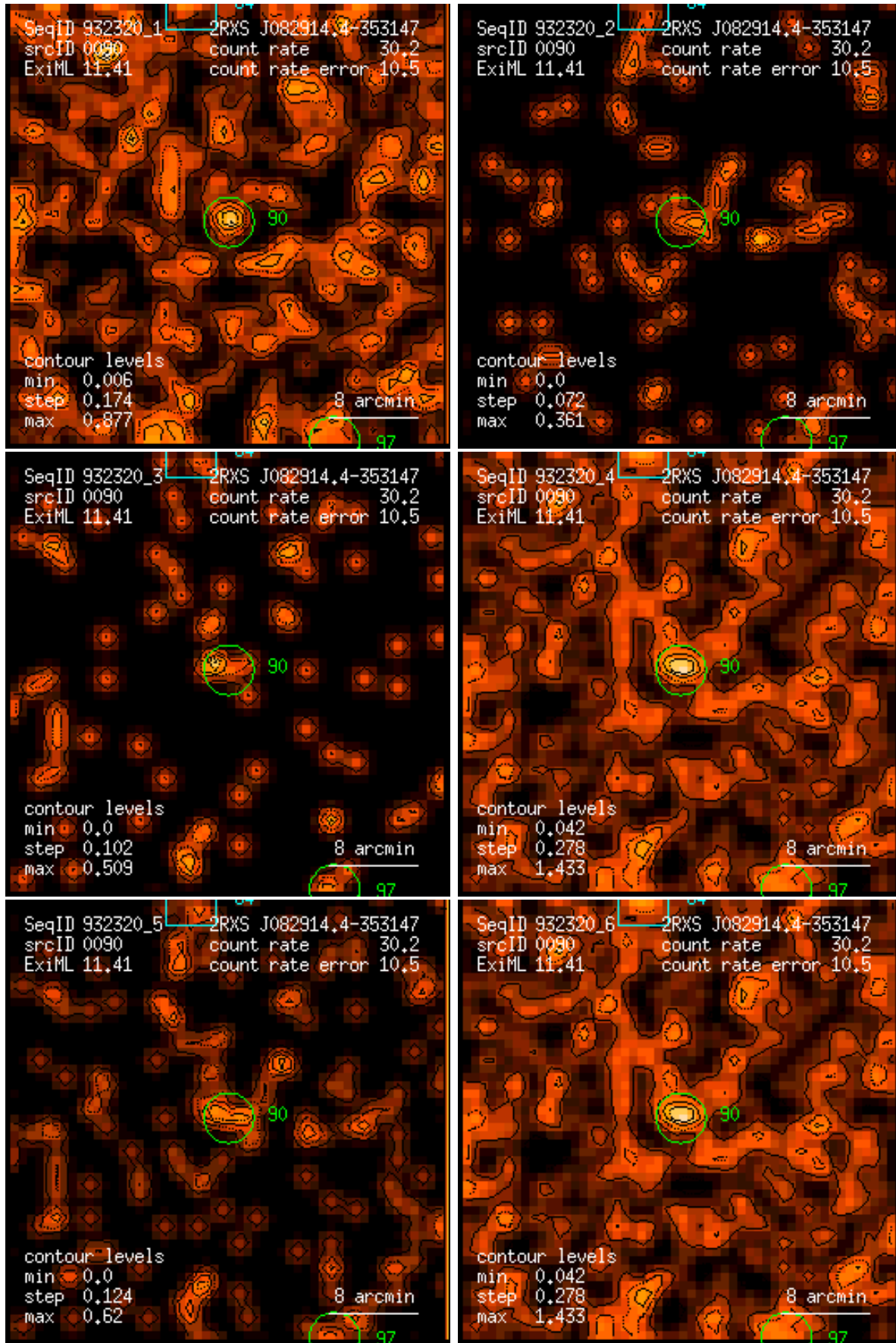
Figure 90: RASS 932320: detection 0090: band rate images, Gaussian filter: (1) PSPPC channels 11 – 41, (2) 52 – 90, (3) 91 – 201, (4) 11 – 235, (5) 52 – 201, (6) 11 – 201. Broad band rates in counts/ks. Band rate contour levels in counts/ks/arcmin 2 .
