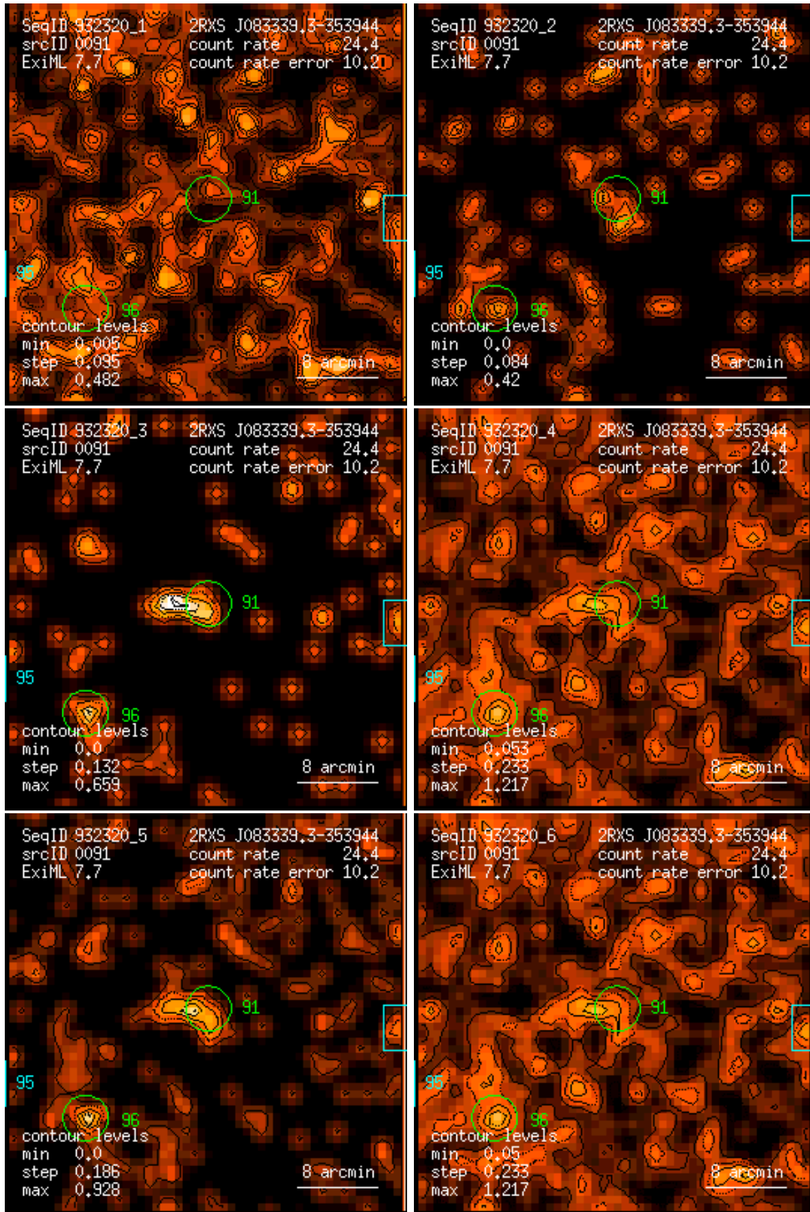
Figure 91: RASS 932320: detection 0091: band rate images, Gaussian filter: (1) PSPC channels 11 – 41, (2) 52 – 90, (3) 91 – 201, (4) 11 – 235, (5) 52 – 201, (6) 11 – 201. Broad band rates in counts/ks. Band rate contour levels in counts/ks/arcmin 2 .
