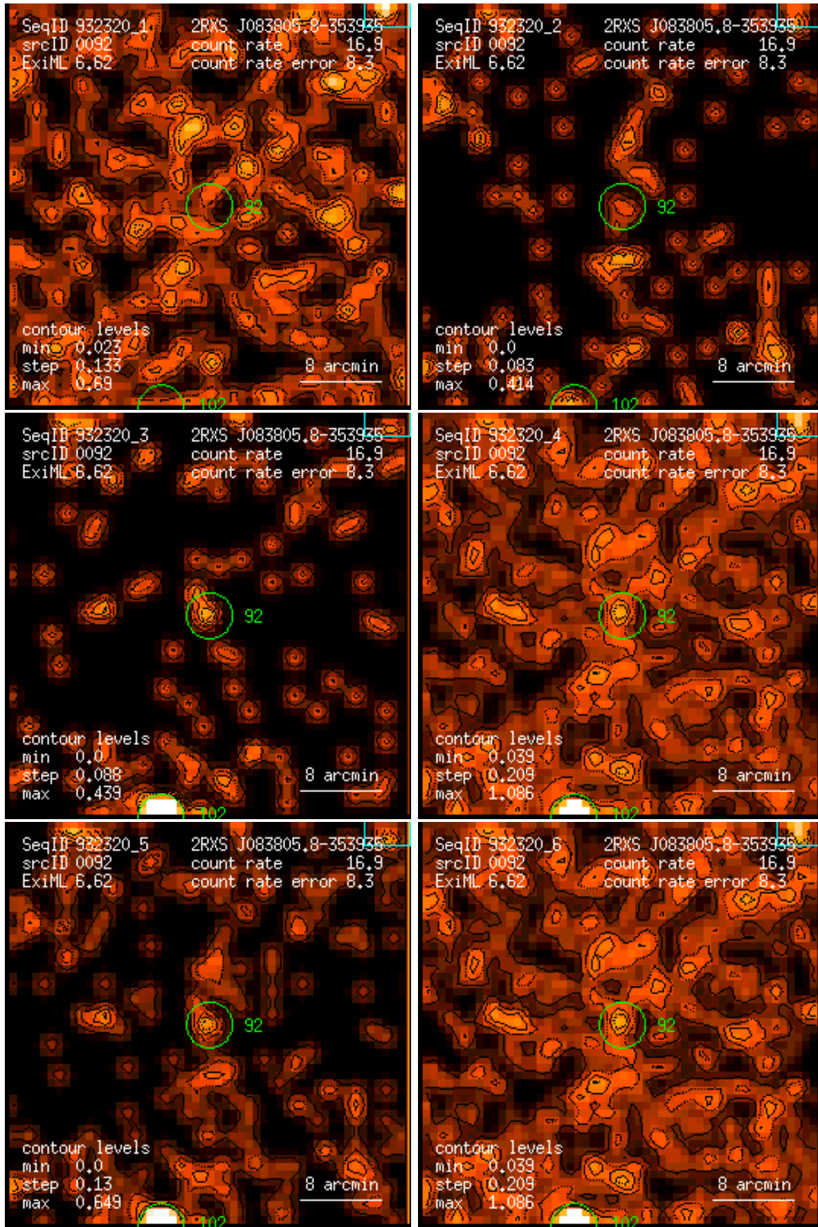
Figure 92: RASS 932320: detection 0092: band rate images, Gaussian filter: (1) PSPC channels 11 – 41, (2) 52 – 90, (3) 91 – 201, (4) 11 – 235, (5) 52 – 201, (6) 11 – 201. Broad band rates in counts/ks. Band rate contour levels in counts/ks/arcmin 2 .
