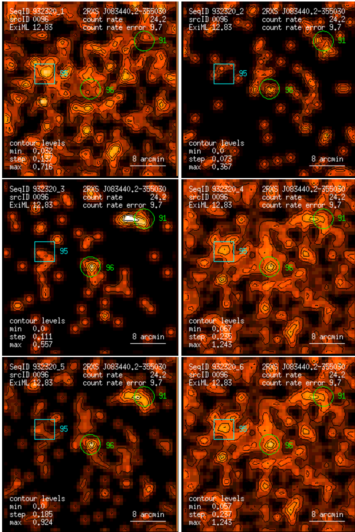
Figure 96: RASS 932320: detection 0096: band rate images, Gaussian filter: (1) PSPC channels 11 – 41, (2) 52 – 90, (3) 91 – 201, (4) 11 – 235, (5) 52 – 201, (6) 11 – 201. Broad band rates in counts/ks. Band rate contour levels in counts/ks/arcmin 2 .
