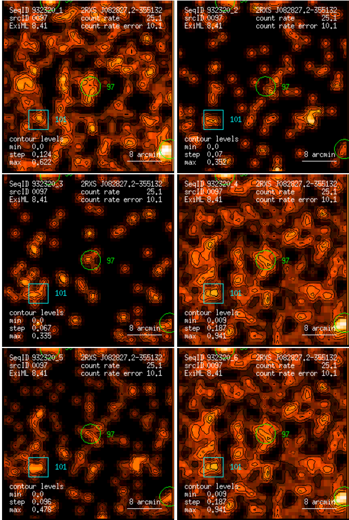
Figure 97: RASS 932320: detection 0097: band rate images, Gaussian filter: (1) PSPC channels 11 – 41, (2) 52 – 90, (3) 91 – 201, (4) 11 – 235, (5) 52 – 201, (6) 11 – 201. Broad band rates in counts/ks. Band rate contour levels in counts/ks/arcmin 2 .
