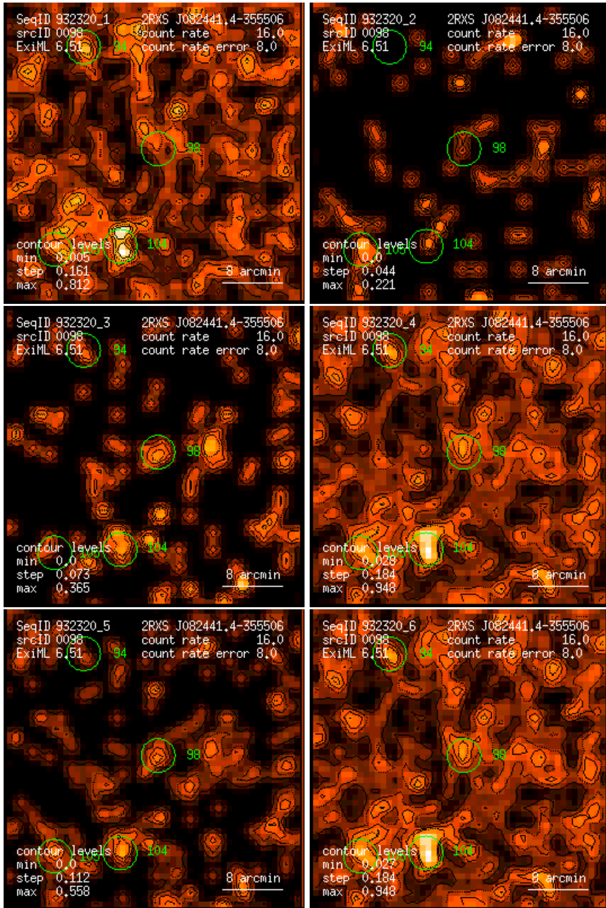
Figure 98: RASS 932320: detection 0098: band rate images, Gaussian filter: (1) PSPC channels 11 – 41, (2) 52 – 90, (3) 91 – 201, (4) 11 – 235, (5) 52 – 201, (6) 11 – 201. Broad band rates in counts/ks. Band rate contour levels in counts/ks/arcmin 2 .
