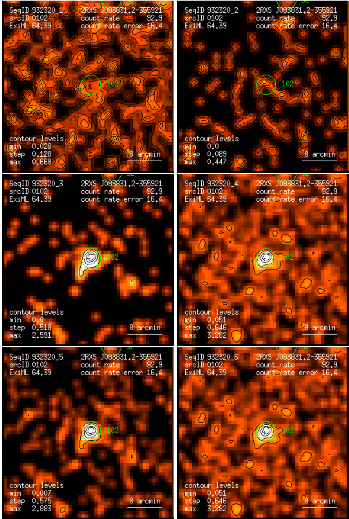
Figure 102: RASS 932320: detection 0102: band rate images, Gaussian filter: (1) PSPC channels 11 – 41, (2) 52 – 90, (3) 91 – 201, (4) 11 – 235, (5) 52 – 201, (6) 11 – 201. Broad band rates in counts/ks. Band rate contour levels in counts/ks/arcmin 2 .
