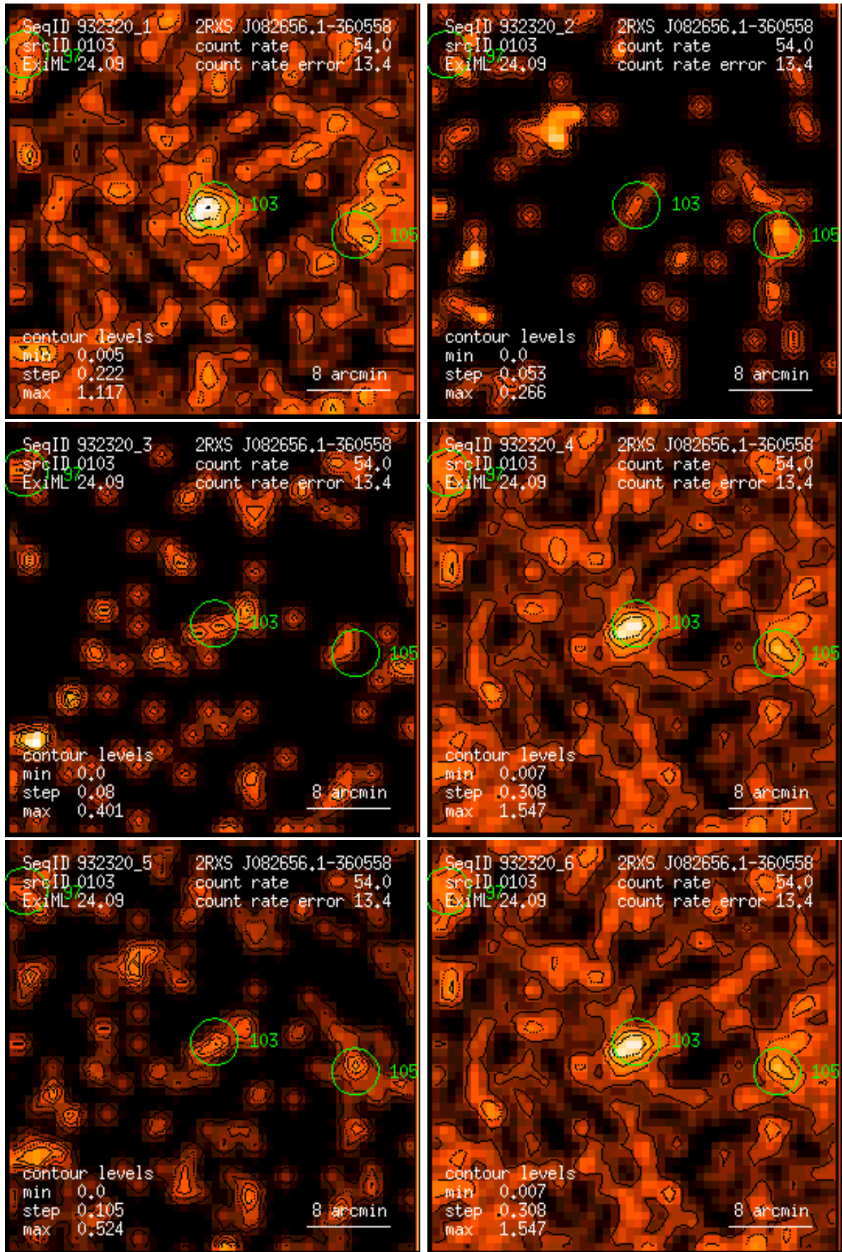
Figure 103: RASS 932320: detection 0103: band rate images, Gaussian filter: (1) PSPC channels 11 – 41, (2) 52 – 90, (3) 91 – 201, (4) 11 – 235, (5) 52 – 201, (6) 11 – 201. Broad band rates in counts/ks. Band rate contour levels in counts/ks/arcmin 2 .
