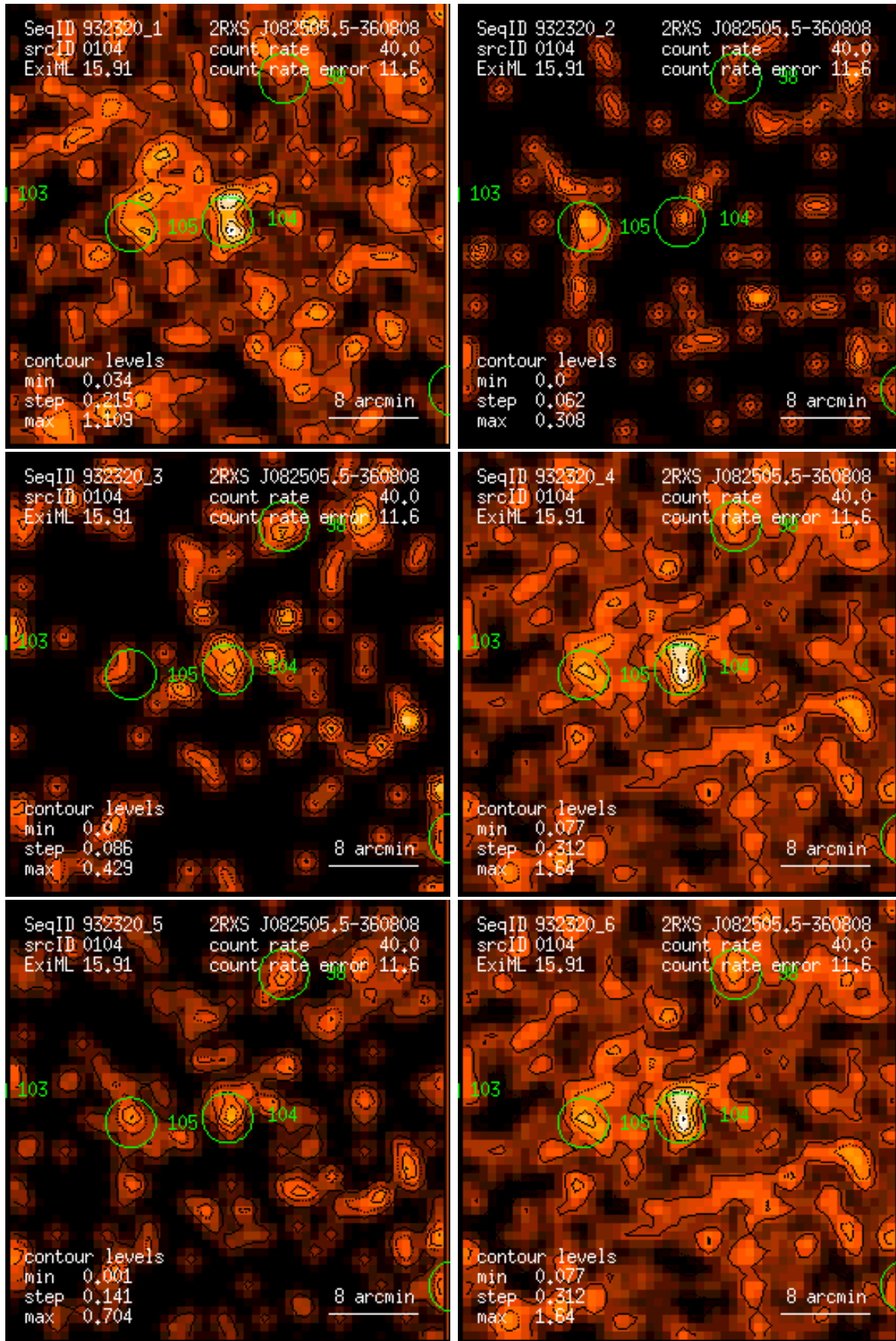
Figure 104: RASS 932320: detection 0104: band rate images, Gaussian filter: (1) PSPC channels 11 – 41, (2) 52 – 90, (3) 91 – 201, (4) 11 – 235, (5) 52 – 201, (6) 11 – 201. Broad band rates in counts/ks. Band rate contour levels in counts/ks/arcmin 2 .
