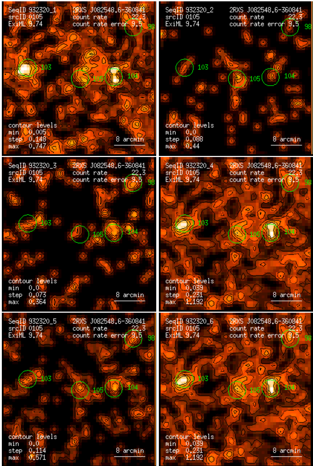
Figure 105: RASS 932320: detection 0105: band rate images, Gaussian filter: (1) PSPC channels 11 – 41, (2) 52 – 90, (3) 91 – 201, (4) 11 – 235, (5) 52 – 201, (6) 11 – 201. Broad band rates in counts/ks. Band rate contour levels in counts/ks/arcmin 2 .
