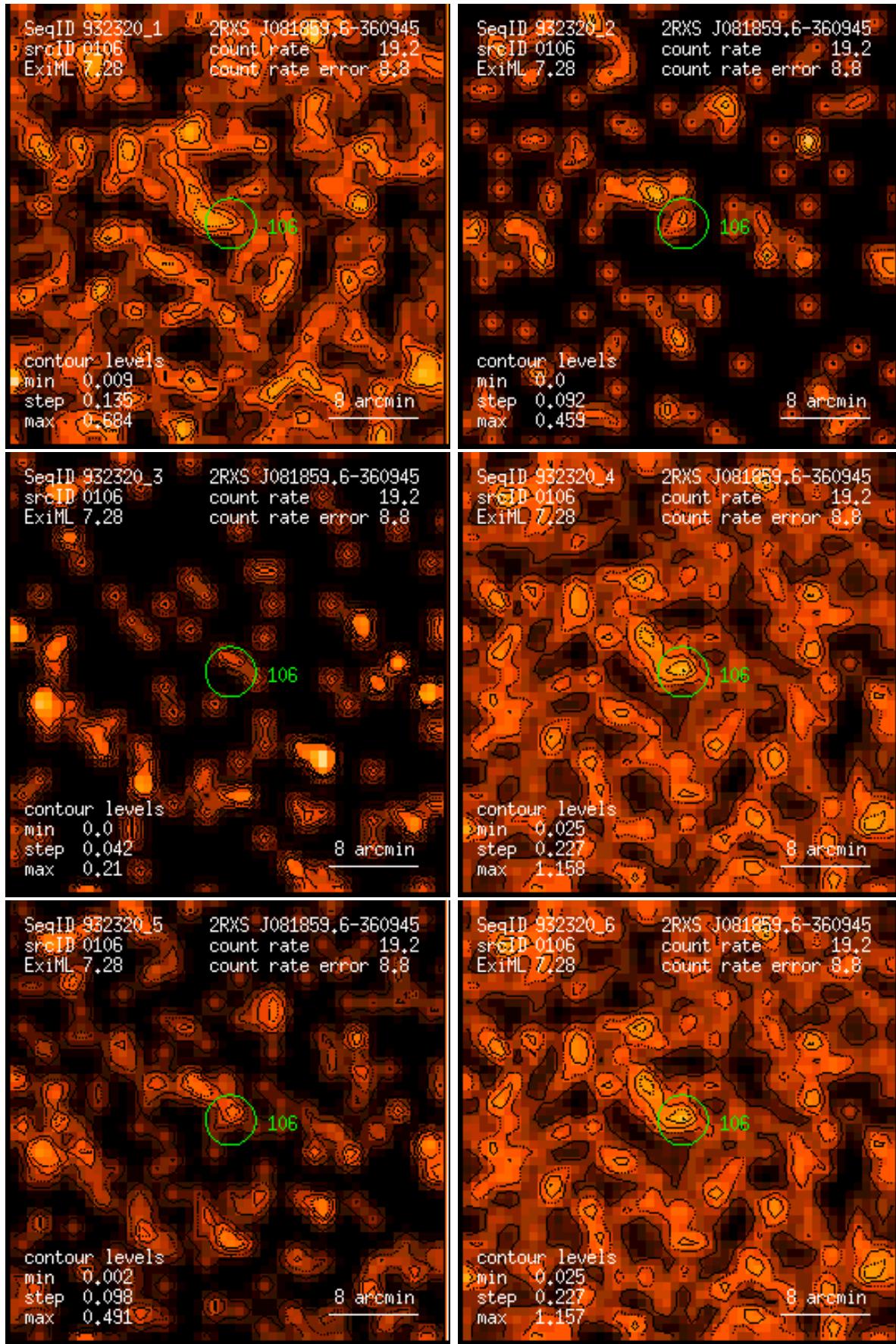
Figure 106: RASS 932320: detection 0106: band rate images, Gaussian filter: (1) PSPC channels 11 – 41, (2) 52 – 90, (3) 91 – 201, (4) 11 – 235, (5) 52 – 201, (6) 11 – 201. Broad band rates in counts/ks. Band rate contour levels in counts/ks/arcmin 2 .
