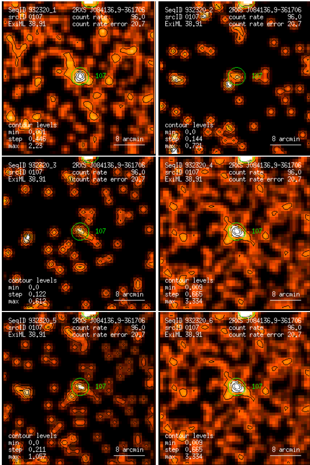
Figure 107: RASS 932320: detection 0107: band rate images, Gaussian filter: (1) PSPC channels 11 – 41, (2) 52 – 90, (3) 91 – 201, (4) 11 – 235, (5) 52 – 201, (6) 11 – 201. Broad band rates in counts/ks. Band rate contour levels in counts/ks/arcmin 2 .
