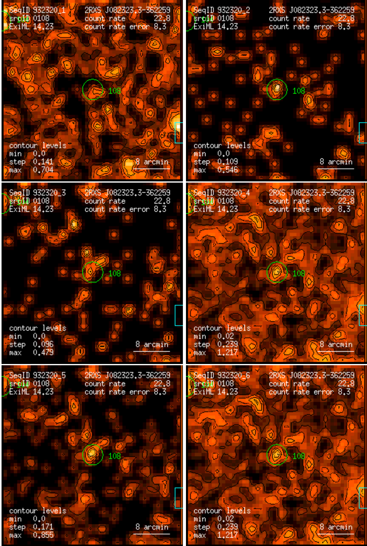
Figure 108: RASS 932320: detection 0108: band rate images, Gaussian filter: (1) PSPC channels 11 – 41, (2) 52 – 90, (3) 91 – 201, (4) 11 – 235, (5) 52 – 201, (6) 11 – 201. Broad band rates in counts/ks. Band rate contour levels in counts/ks/arcmin 2 .
