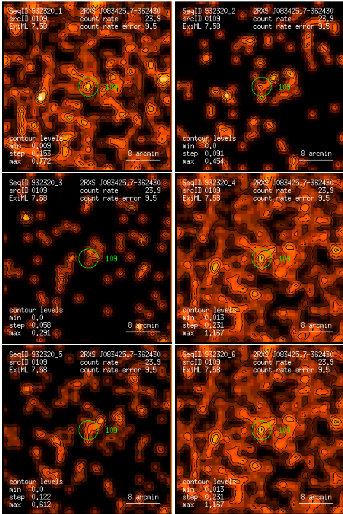
Figure 109: RASS 932320: detection 0109: band rate images, Gaussian filter: (1) PSPC channels 11 – 41, (2) 52 – 90, (3) 91 – 201, (4) 11 – 235, (5) 52 – 201, (6) 11 – 201. Broad band rates in counts/ks. Band rate contour levels in counts/ks/arcmin 2 .
