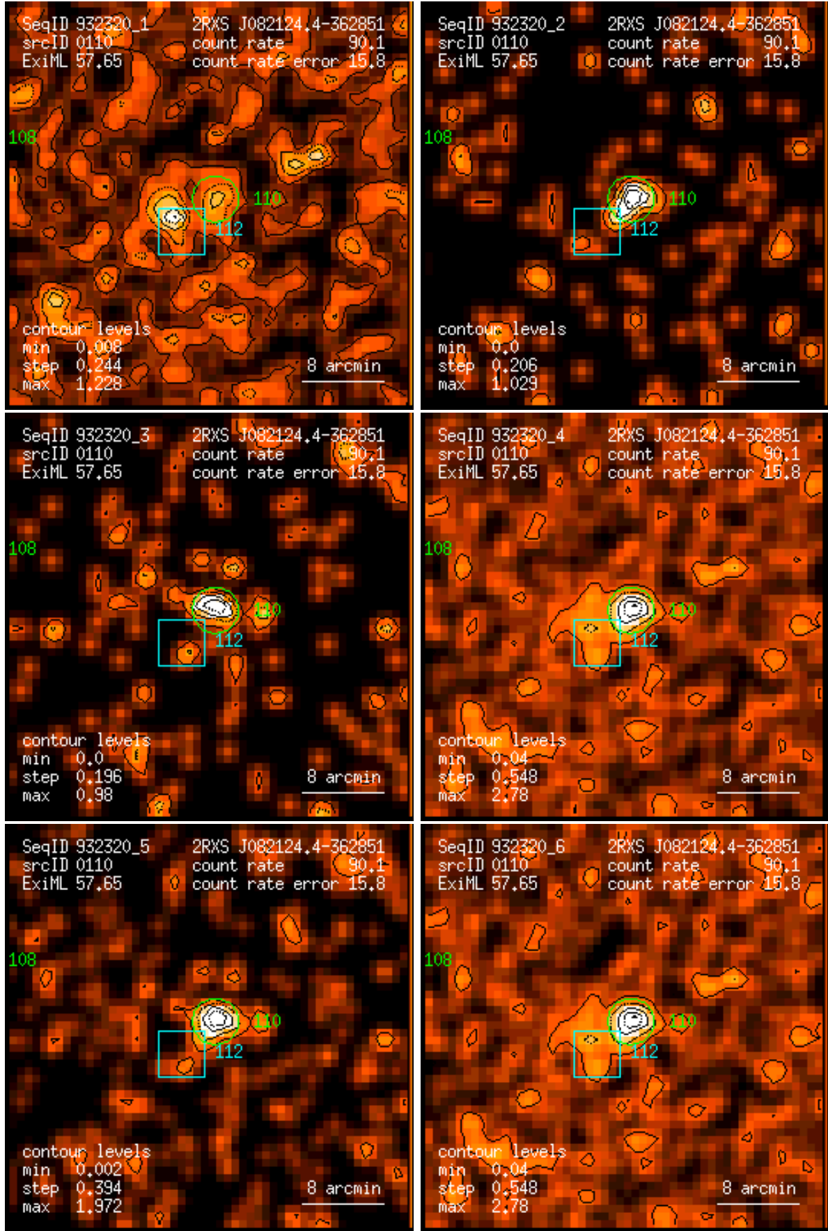
Figure 110: RASS 932320: detection 0110: band rate images, Gaussian filter: (1) PSPC channels 11 – 41, (2) 52 – 90, (3) 91 – 201, (4) 11 – 235, (5) 52 – 201, (6) 11 – 201. Broad band rates in counts/ks. Band rate contour levels in counts/ks/arcmin 2 .
