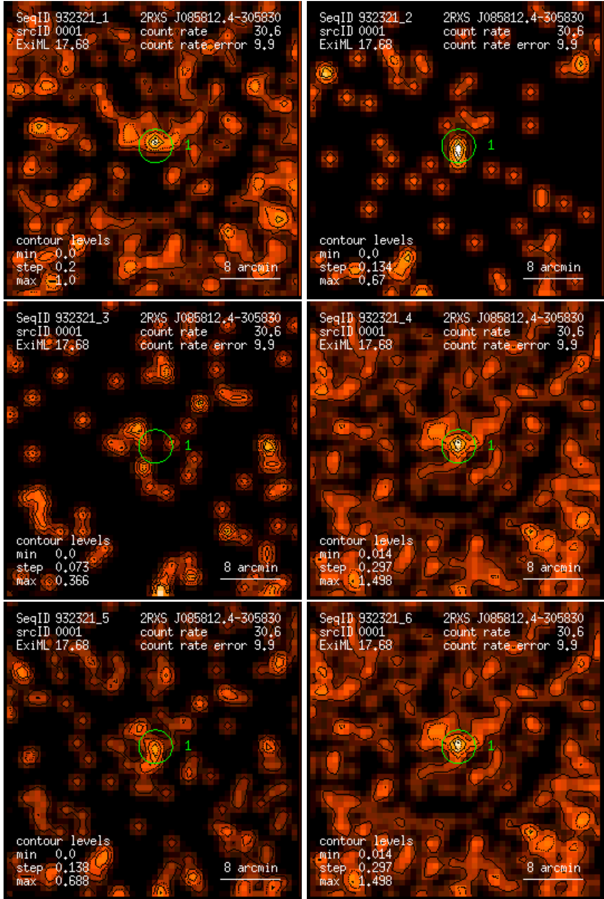
Figure 1: RASS 932321: detection 0001: band rate images, Gaussian filter: (1) PSPC channels 11 – 41, (2) 52 – 90, (3) 91 – 201, (4) 11 – 235, (5) 52 – 201, (6) 11 – 201. Broad band rates in counts/ks. Band rate contour levels in counts/ks/arcmin 2 .
