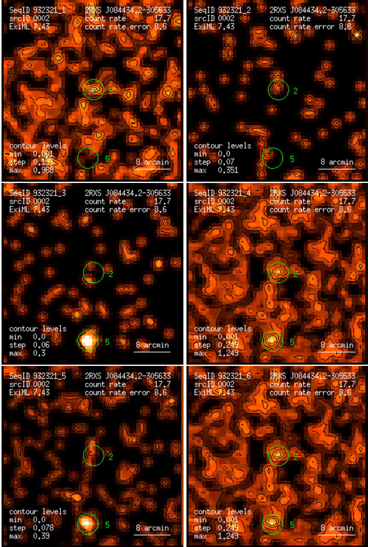
Figure 2: RASS 932321: detection 0002: band rate images, Gaussian filter: (1) PSPC channels 11 – 41, (2) 52 – 90, (3) 91 – 201, (4) 11 – 235, (5) 52 – 201, (6) 11 – 201. Broad band rates in counts/ks. Band rate contour levels in counts/ks/arcmin 2 .
