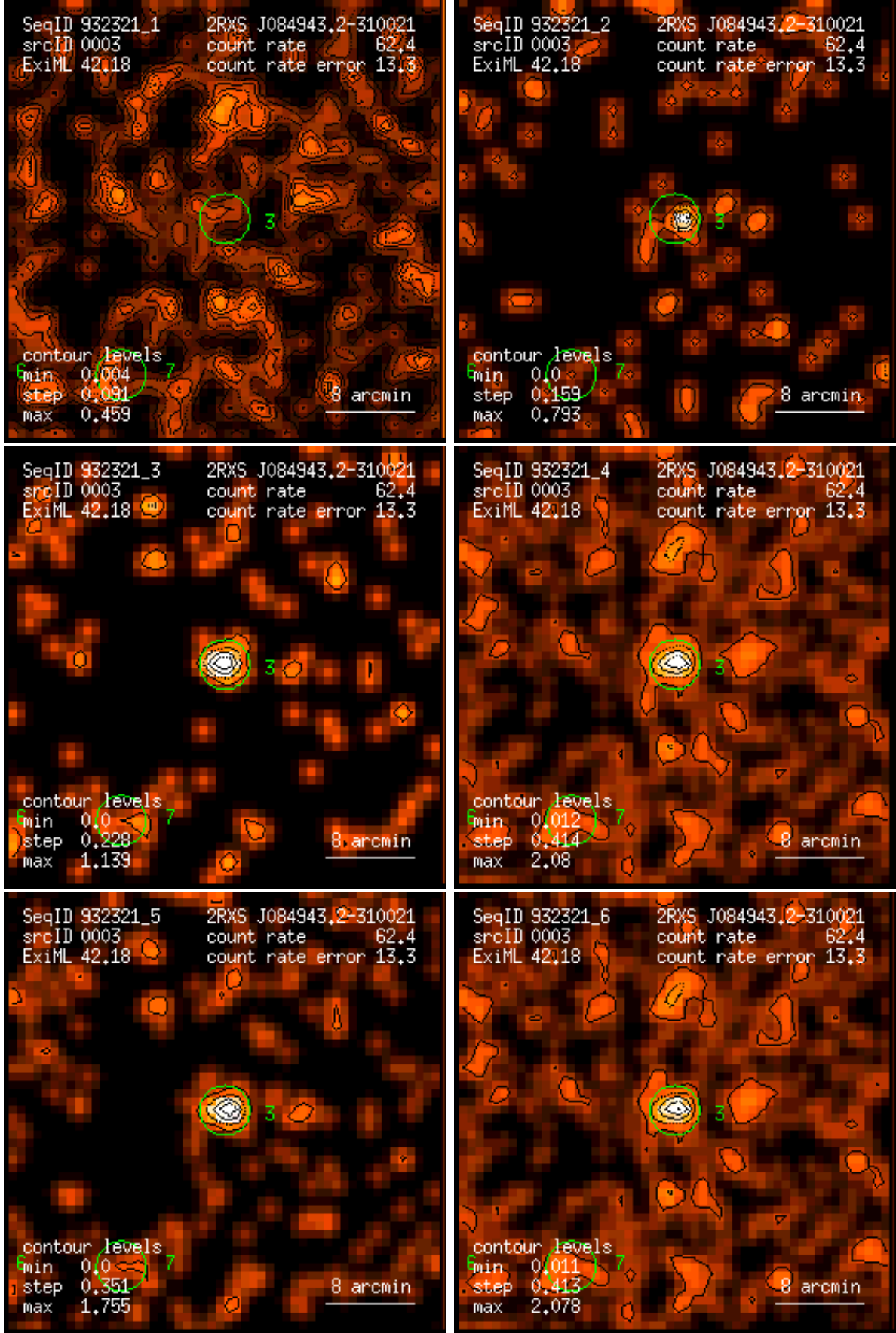
Figure 3: RASS 932321: detection 0003: band rate images, Gaussian filter: (1) PSPC channels 11 – 41, (2) 52 – 90, (3) 91 – 201, (4) 11 – 235, (5) 52 – 201, (6) 11 – 201. Broad band rates in counts/ks. Band rate contour levels in counts/ks/arcmin 2 .
