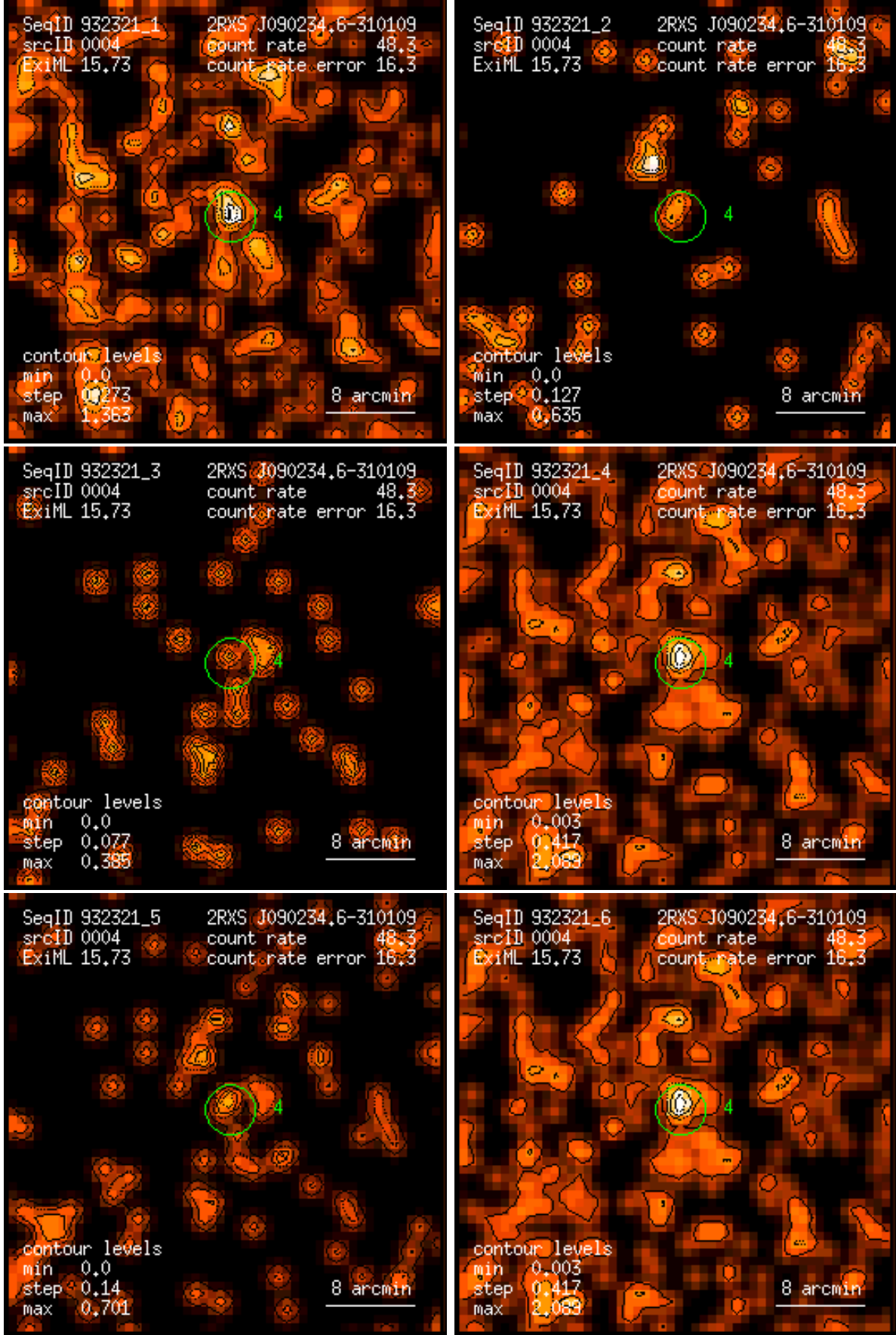
Figure 4: RASS 932321: detection 0004: band rate images, Gaussian filter: (1) PSPC channels 11 – 41, (2) 52 – 90, (3) 91 – 201, (4) 11 – 235, (5) 52 – 201, (6) 11 – 201. Broad band rates in counts/ks. Band rate contour levels in counts/ks/arcmin 2 .
