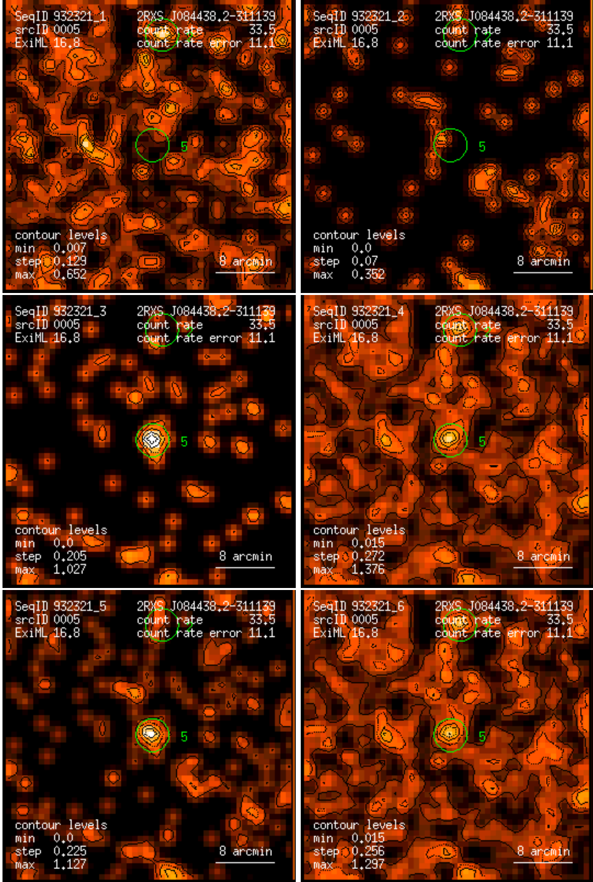
Figure 5: RASS 932321: detection 0005: band rate images, Gaussian filter: (1) PSPC channels 11 – 41, (2) 52 – 90, (3) 91 – 201, (4) 11 – 235, (5) 52 – 201, (6) 11 – 201. Broad band rates in counts/ks. Band rate contour levels in counts/ks/arcmin 2 .
