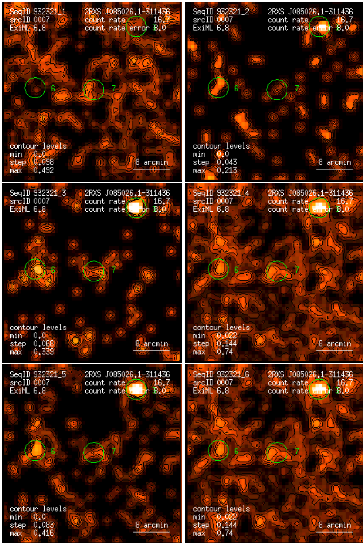
Figure 7: RASS 932321: detection 0007: band rate images, Gaussian filter: (1) PSPC channels 11 – 41, (2) 52 – 90, (3) 91 – 201, (4) 11 – 235, (5) 52 – 201, (6) 11 – 201. Broad band rates in counts/ks. Band rate contour levels in counts/ks/arcmin 2 .
