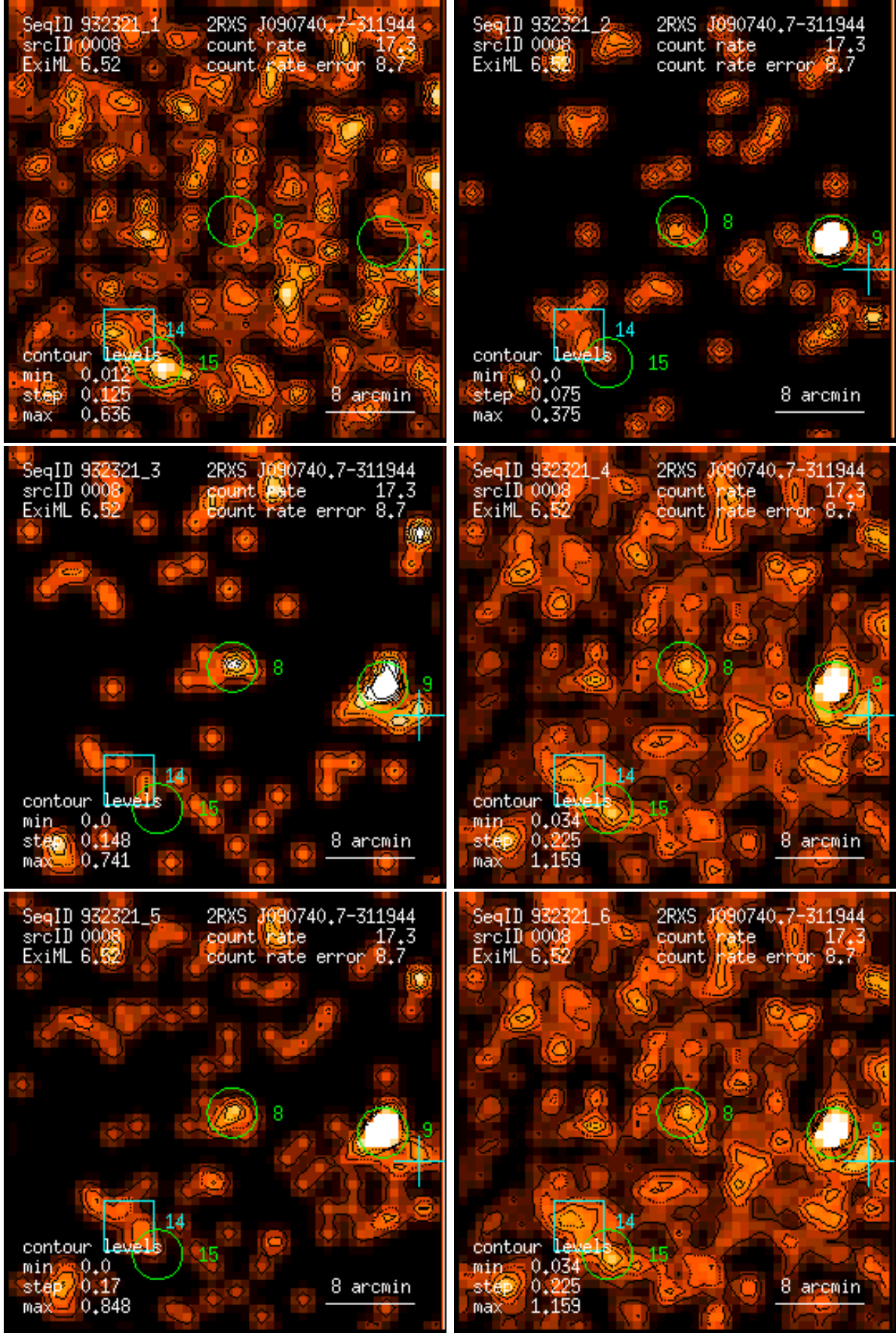
Figure 8: RASS 932321: detection 0008: band rate images, Gaussian filter: (1) PSPC channels 11 – 41, (2) 52 – 90, (3) 91 – 201, (4) 11 – 235, (5) 52 – 201, (6) 11 – 201. Broad band rates in counts/ks. Band rate contour levels in counts/ks/arcmin 2 .
