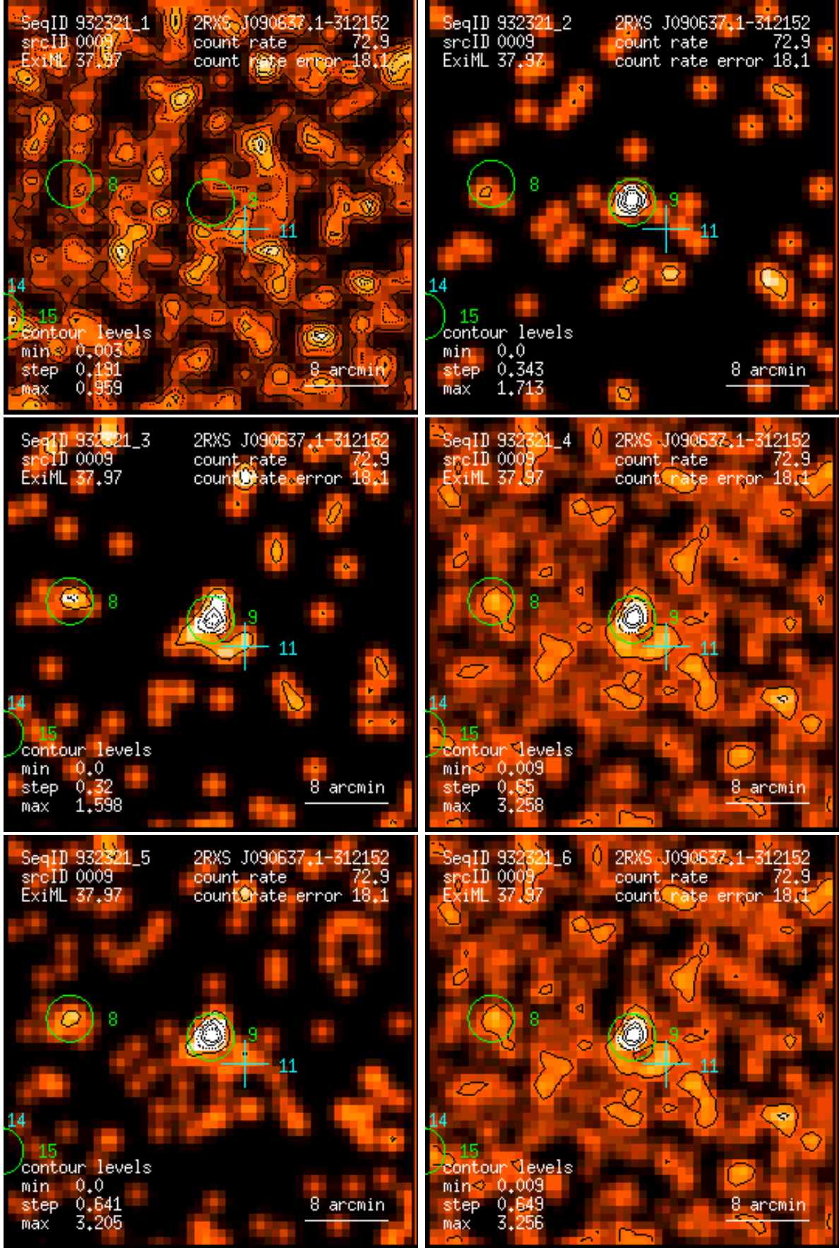
Figure 9: RASS 932321: detection 0009: band rate images, Gaussian filter: (1) PSPC channels 11 – 41, (2) 52 – 90, (3) 91 – 201, (4) 11 – 235, (5) 52 – 201, (6) 11 – 201. Broad band rates in counts/ks. Band rate contour levels in counts/ks/arcmin 2 .
