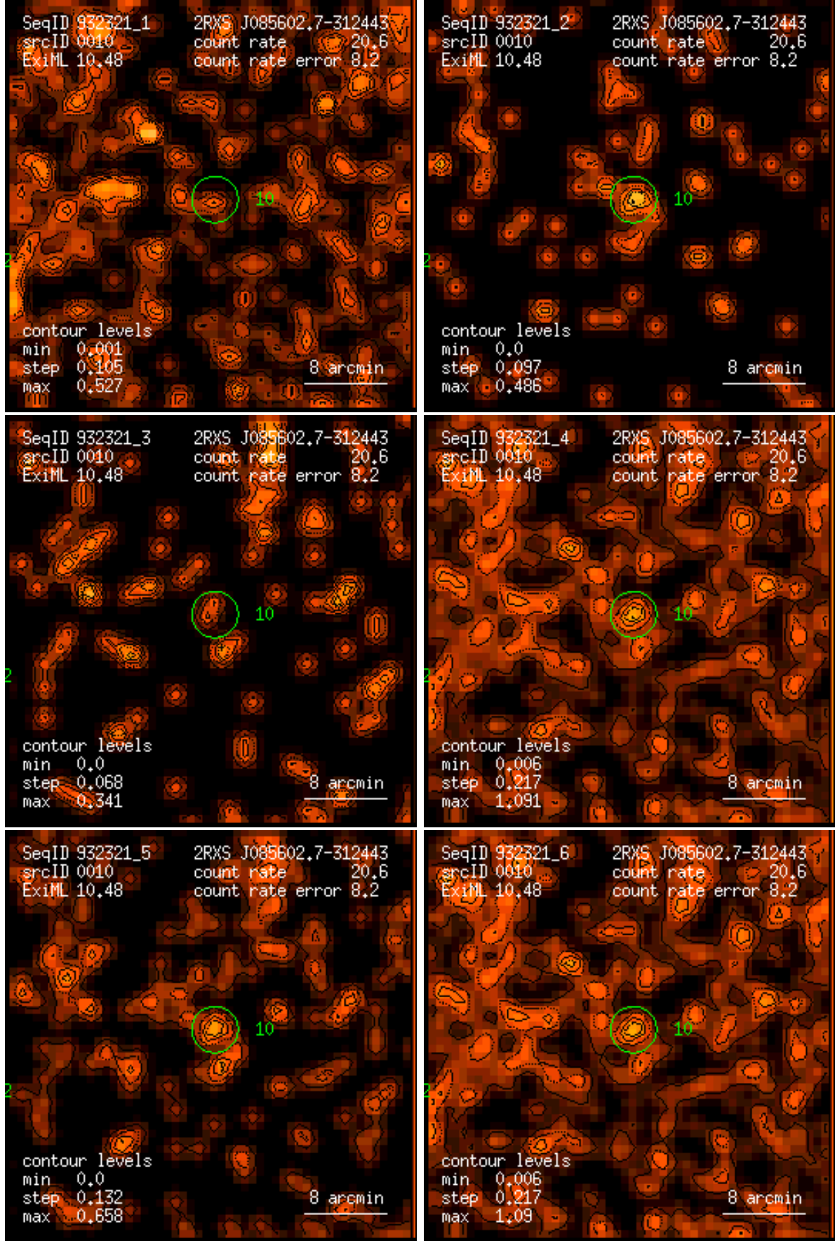
Figure 10: RASS 932321: detection 0010: band rate images, Gaussian filter: (1) PSPC channels 11 – 41, (2) 52 – 90, (3) 91 – 201, (4) 11 – 235, (5) 52 – 201, (6) 11 – 201. Broad band rates in counts/ks. Band rate contour levels in counts/ks/arcmin 2 .
