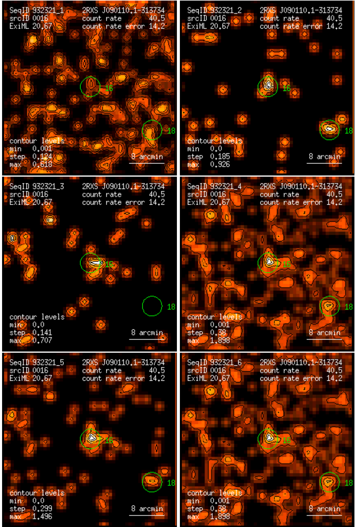
Figure 16: RASS 932321: detection 0016: band rate images, Gaussian filter: (1) PSPC channels 11 – 41, (2) 52 – 90, (3) 91 – 201, (4) 11 – 235, (5) 52 – 201, (6) 11 – 201. Broad band rates in counts/ks. Band rate contour levels in counts/ks/arcmin 2 .
