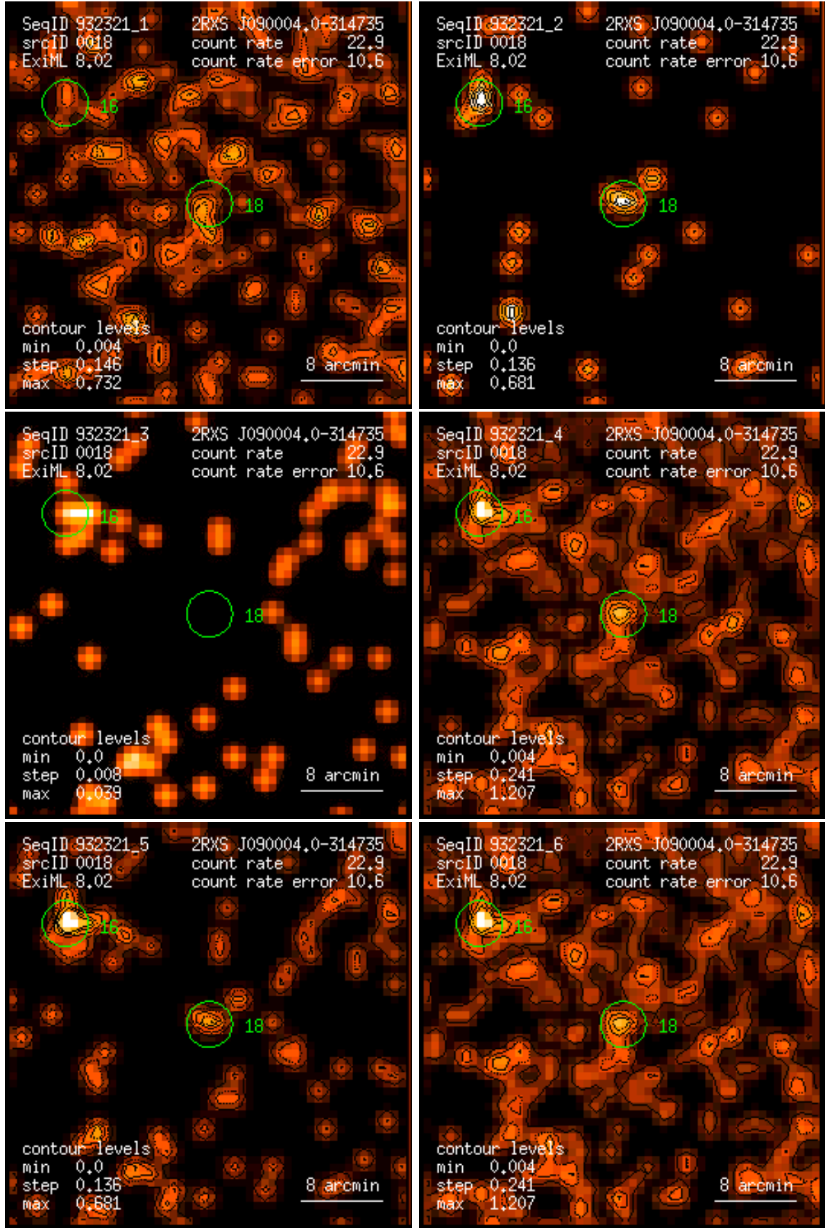
Figure 18: RASS 932321: detection 0018: band rate images, Gaussian filter: (1) PSPC channels 11 – 41, (2) 52 – 90, (3) 91 – 201, (4) 11 – 235, (5) 52 – 201, (6) 11 – 201. Broad band rates in counts/ks. Band rate contour levels in counts/ks/arcmin 2 .
