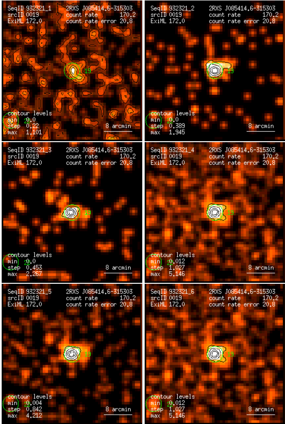
Figure 19: RASS 932321: detection 0019: band rate images, Gaussian filter: (1) PSPC channels 11 – 41, (2) 52 – 90, (3) 91 – 201, (4) 11 – 235, (5) 52 – 201, (6) 11 – 201. Broad band rates in counts/ks. Band rate contour levels in counts/ks/arcmin 2 .
